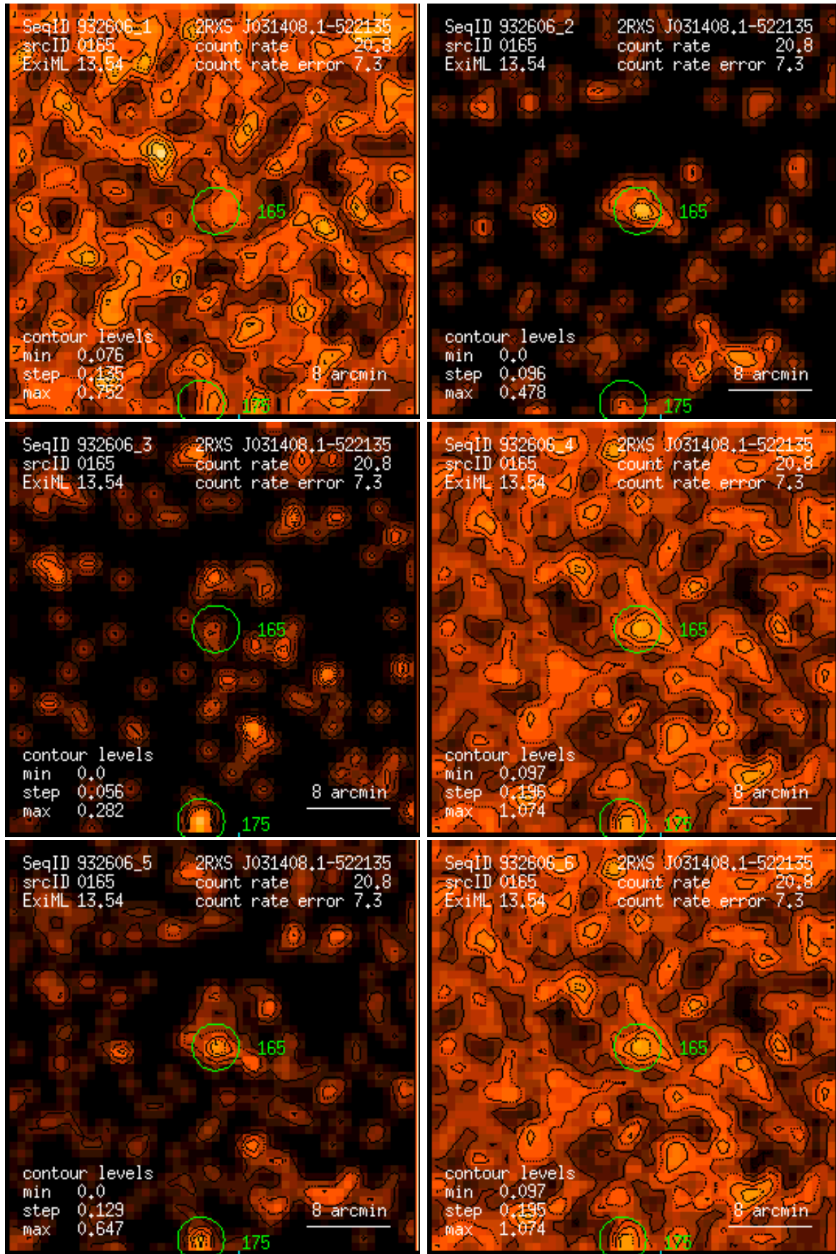
Figure 165: RASS 932606: detection 0165: band rate images, Gaussian filter: (1) PSPC channels 11 – 41, (2) 52 – 90, (3) 91 – 201, (4) 11 – 235, (5) 52 – 201, (6) 11 – 201. Broad band rates in counts/ks. Band rate contour levels in counts/ks/arcmin 2 .
