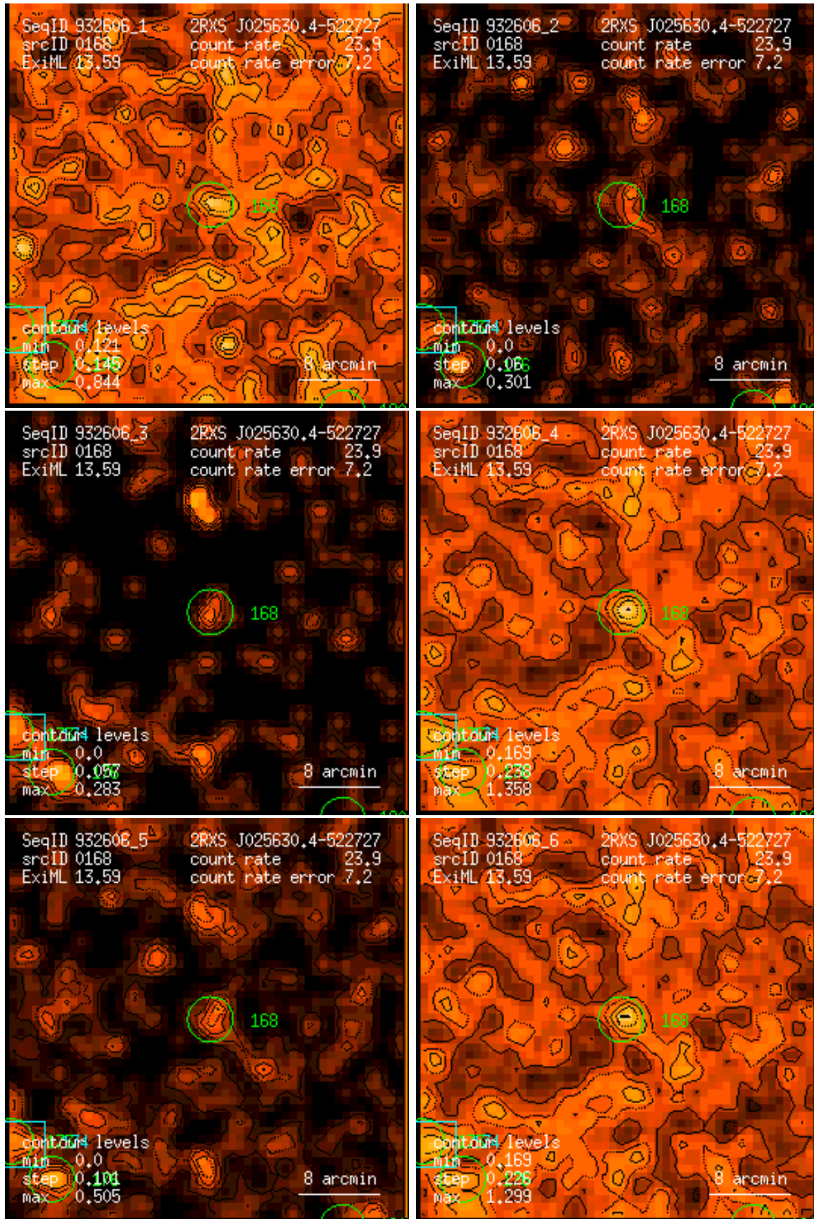
Figure 168: RASS 932606: detection 0168: band rate images, Gaussian filter: (1) PSPC channels 11 – 41, (2) 52 – 90, (3) 91 – 201, (4) 11 – 235, (5) 52 – 201, (6) 11 – 201. Broad band rates in counts/ks. Band rate contour levels in counts/ks/arcmin 2 .
