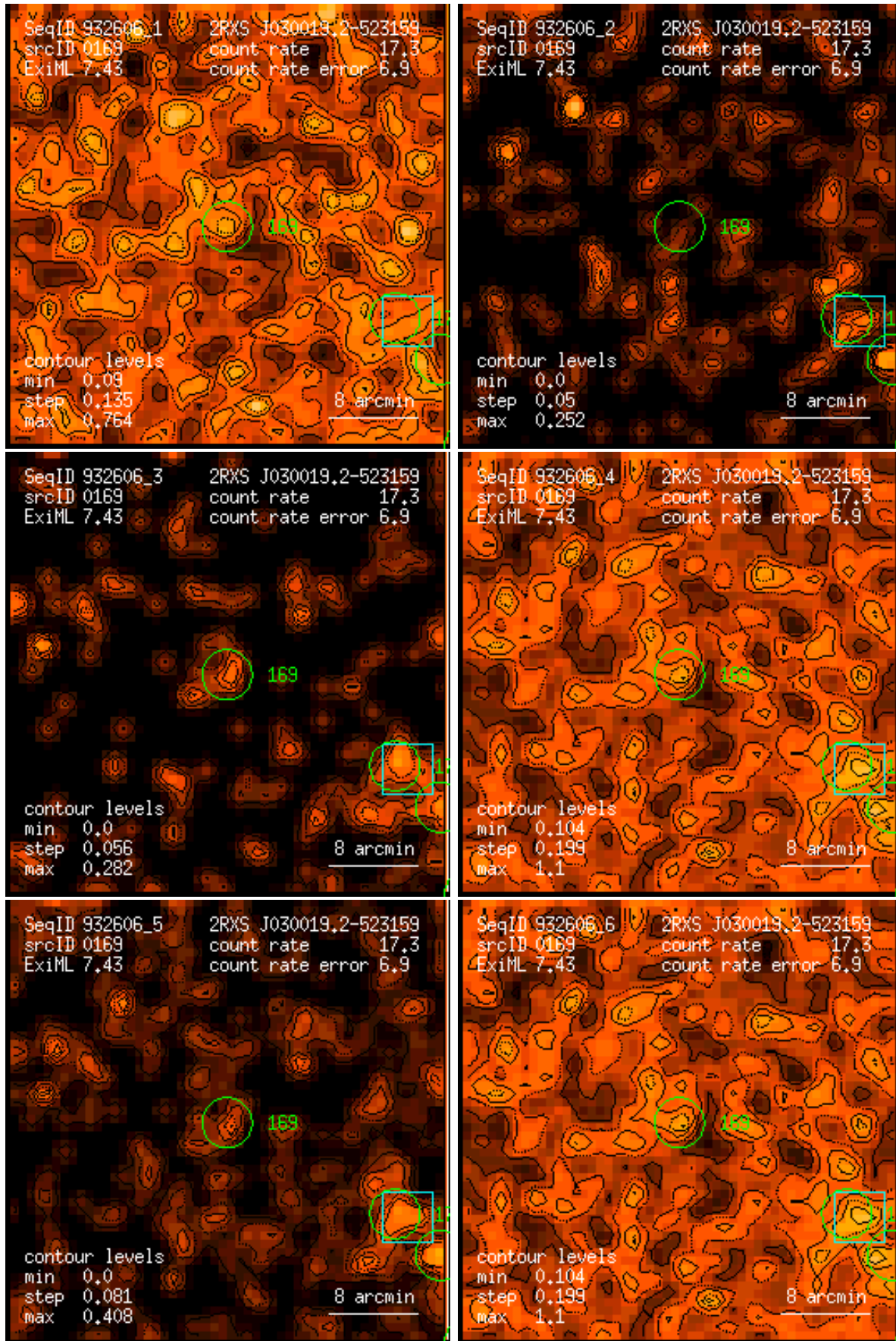
Figure 169: RASS 932606: detection 0169: band rate images, Gaussian filter: (1) PSPC channels 11 – 41, (2) 52 – 90, (3) 91 – 201, (4) 11 – 235, (5) 52 – 201, (6) 11 – 201. Broad band rates in counts/ks. Band rate contour levels in counts/ks/arcmin 2 .
