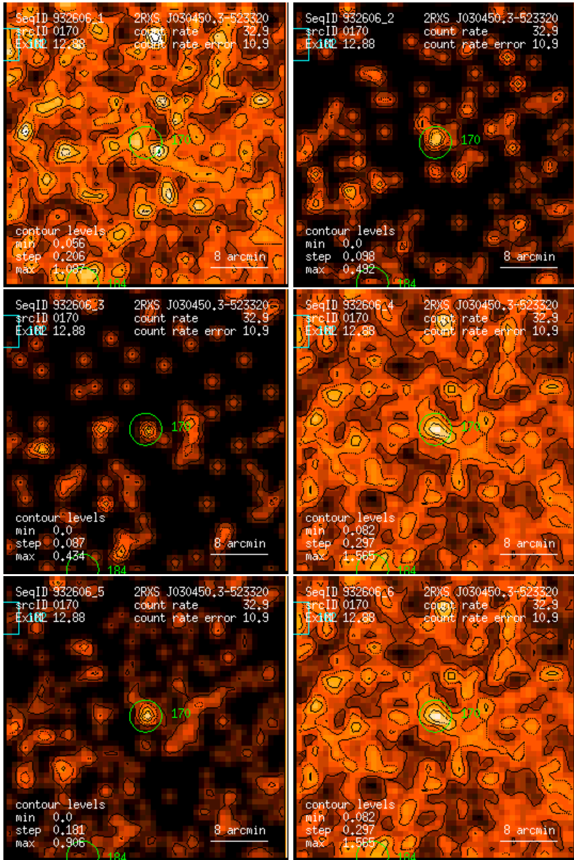
Figure 170: RASS 932606: detection 0170: band rate images, Gaussian filter: (1) PSPC channels 11 – 41, (2) 52 – 90, (3) 91 – 201, (4) 11 – 235, (5) 52 – 201, (6) 11 – 201. Broad band rates in counts/ks. Band rate contour levels in counts/ks/arcmin 2 .
