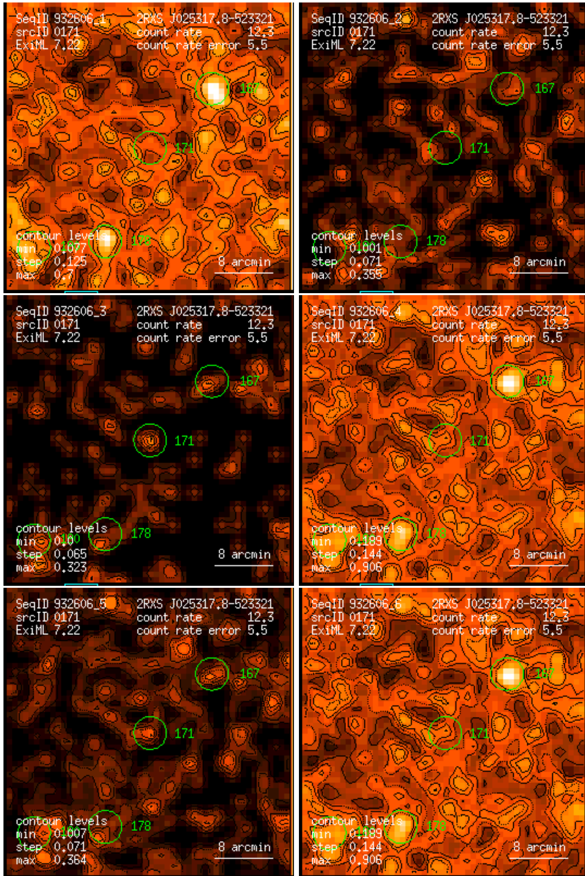
Figure 171: RASS 932606: detection 0171: band rate images, Gaussian filter: (1) PSPC channels 11 – 41, (2) 52 – 90, (3) 91 – 201, (4) 11 – 235, (5) 52 – 201, (6) 11 – 201. Broad band rates in counts/ks. Band rate contour levels in counts/ks/arcmin 2 .
