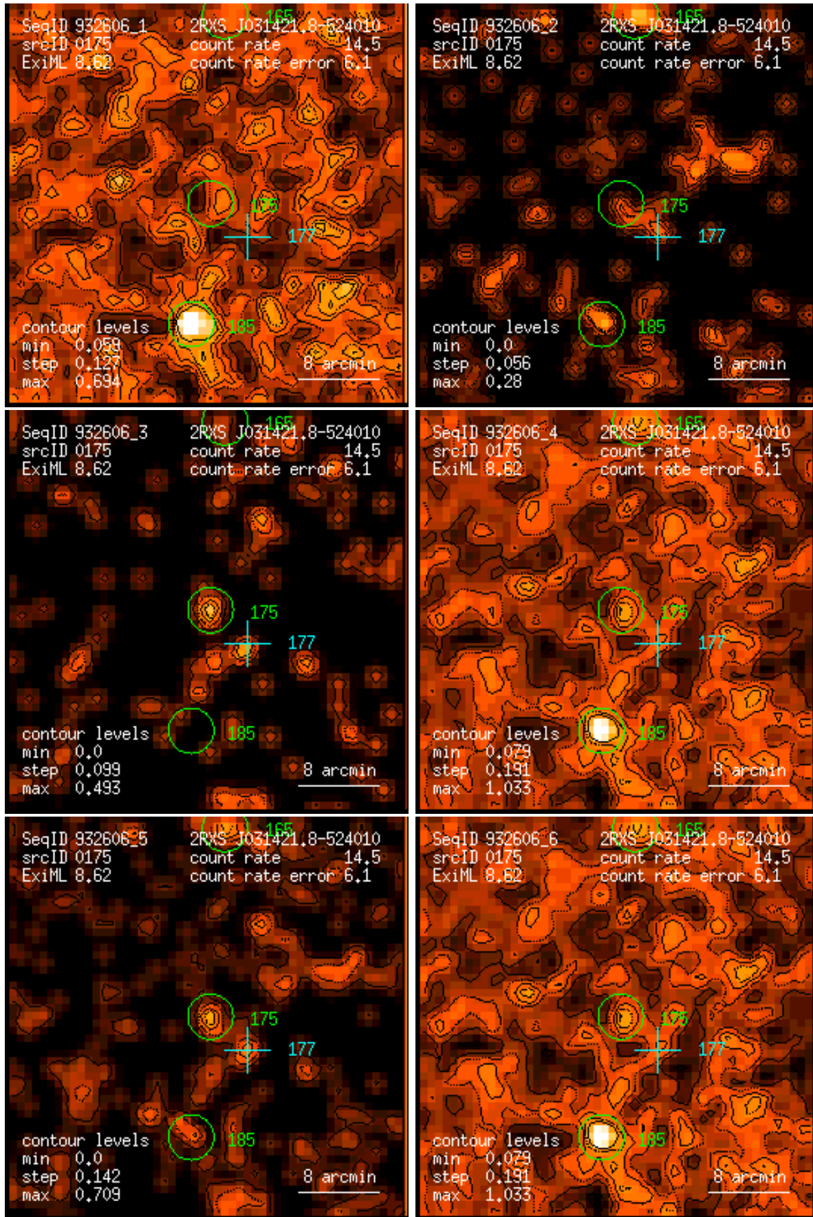
Figure 175: RASS 932606: detection 0175: band rate images, Gaussian filter: (1) PSPC channels 11 – 41, (2) 52 – 90, (3) 91 – 201, (4) 11 – 235, (5) 52 – 201, (6) 11 – 201. Broad band rates in counts/ks. Band rate contour levels in counts/ks/arcmin 2 .
