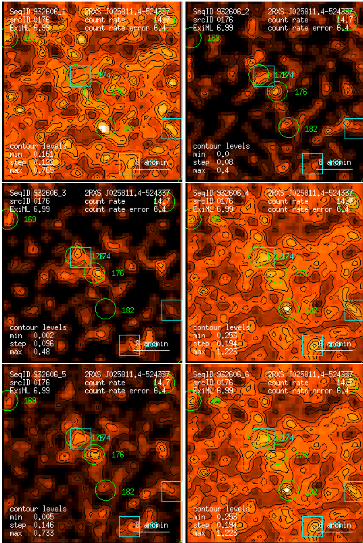
Figure 176: RASS 932606: detection 0176: band rate images, Gaussian filter: (1) PSPC channels 11 – 41, (2) 52 – 90, (3) 91 – 201, (4) 11 – 235, (5) 52 – 201, (6) 11 – 201. Broad band rates in counts/ks. Band rate contour levels in counts/ks/arcmin 2 .
