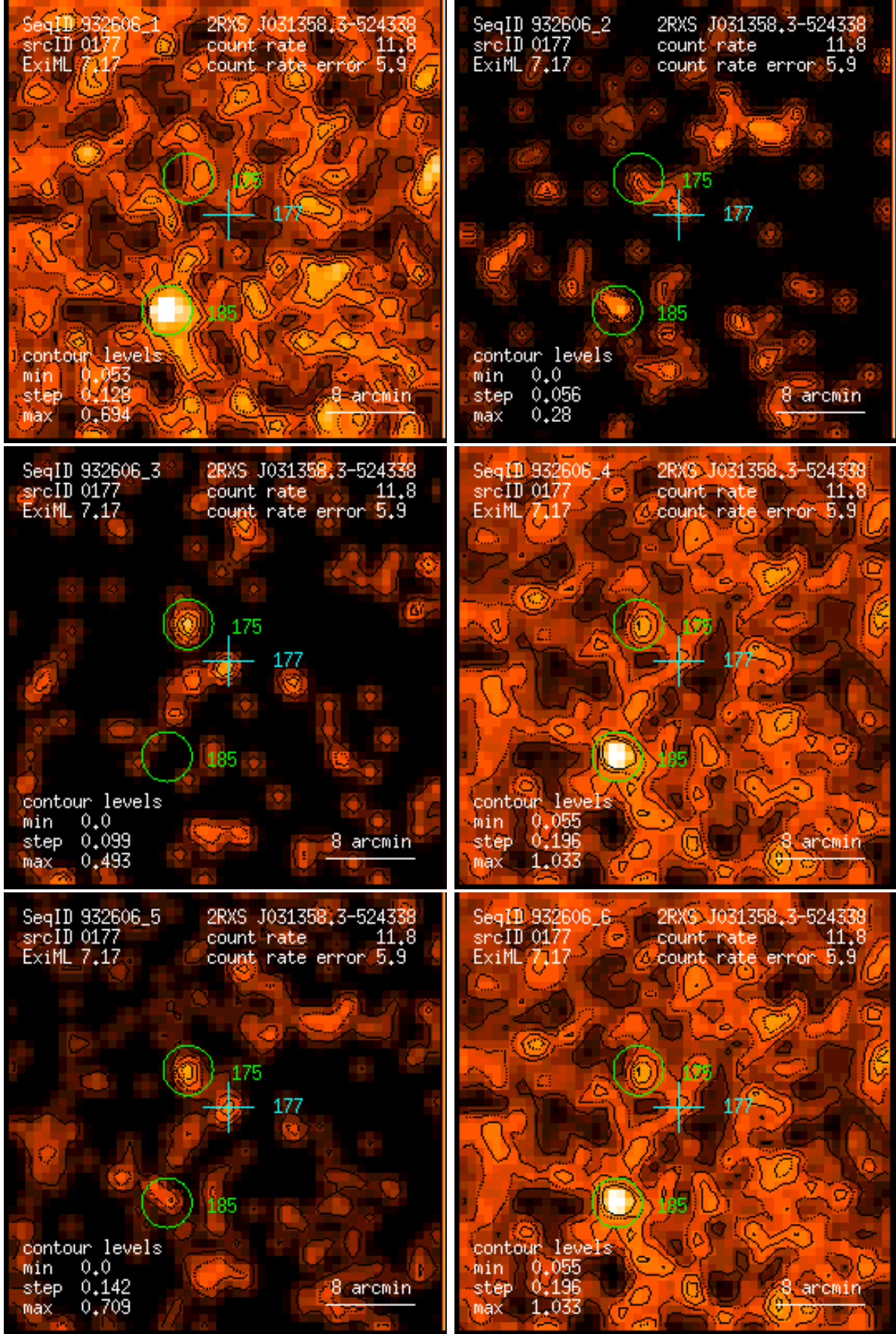
Figure 177: RASS 932606: detection 0177: band rate images, Gaussian filter: (1) PSPC channels 11 – 41, (2) 52 – 90, (3) 91 – 201, (4) 11 – 235, (5) 52 – 201, (6) 11 – 201. Broad band rates in counts/ks. Band rate contour levels in counts/ks/arcmin 2 .
