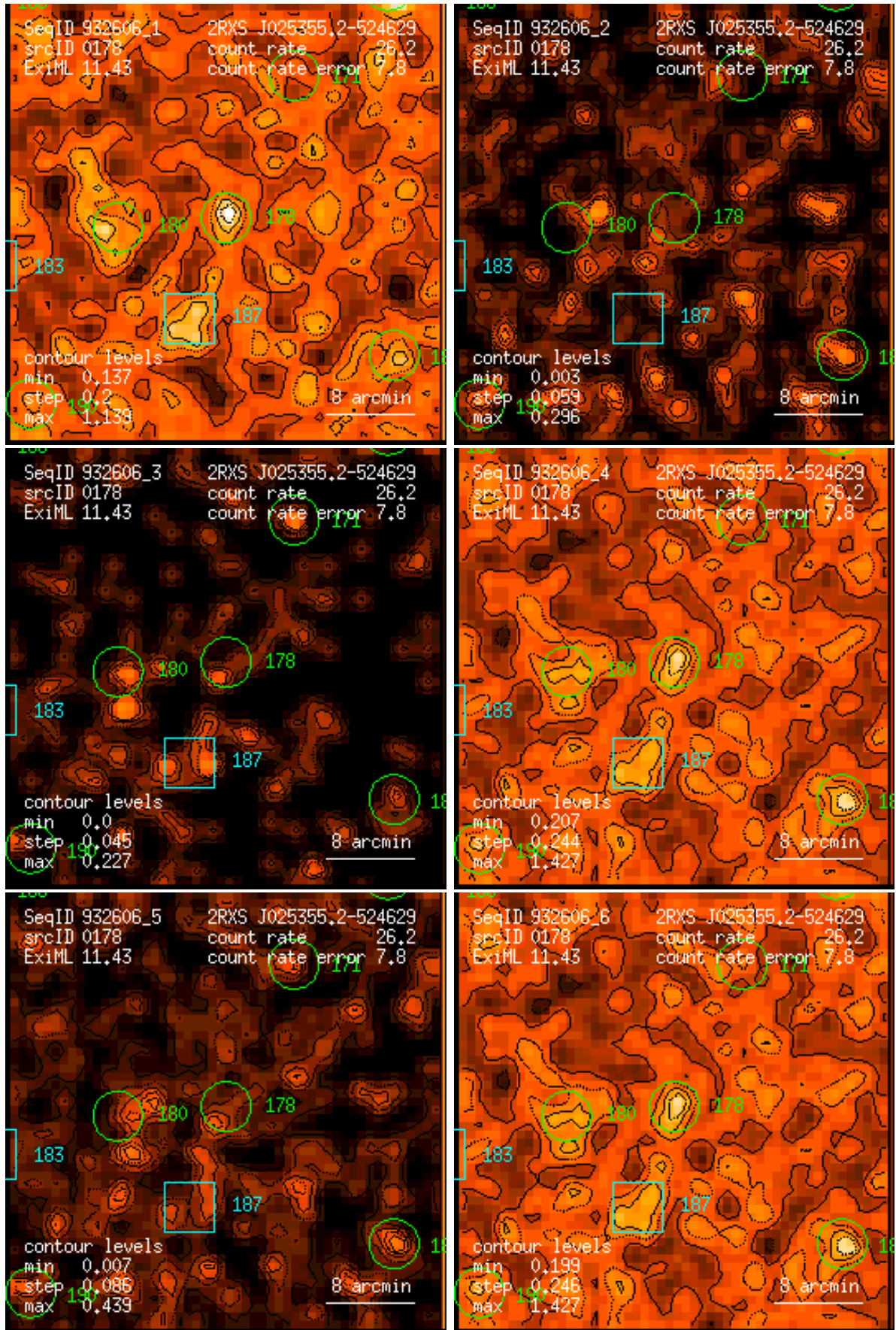
Figure 178: RASS 932606: detection 0178: band rate images, Gaussian filter: (1) PSPC channels 11 – 41, (2) 52 – 90, (3) 91 – 201, (4) 11 – 235, (5) 52 – 201, (6) 11 – 201. Broad band rates in counts/ks. Band rate contour levels in counts/ks/arcmin 2 .
