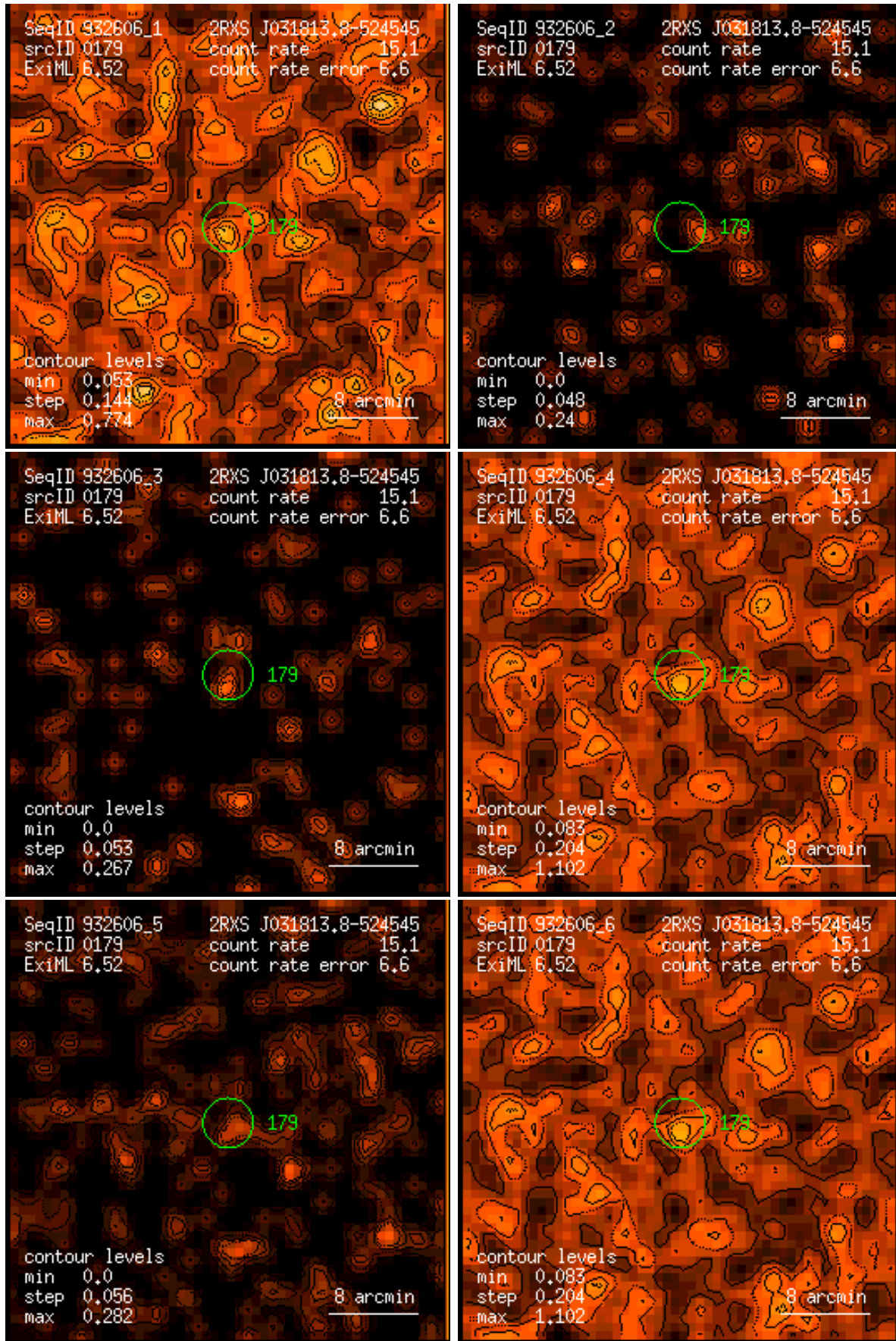
Figure 179: RASS 932606: detection 0179: band rate images, Gaussian filter: (1) PSPC channels 11 – 41, (2) 52 – 90, (3) 91 – 201, (4) 11 – 235, (5) 52 – 201, (6) 11 – 201. Broad band rates in counts/ks. Band rate contour levels in counts/ks/arcmin 2 .
