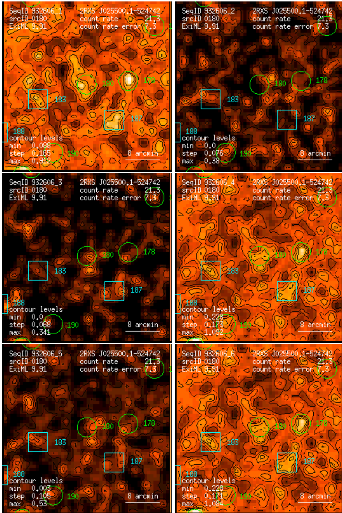
Figure 180: RASS 932606: detection 0180: band rate images, Gaussian filter: (1) PSPC channels 11 – 41, (2) 52 – 90, (3) 91 – 201, (4) 11 – 235, (5) 52 – 201, (6) 11 – 201. Broad band rates in counts/ks. Band rate contour levels in counts/ks/arcmin 2 .
