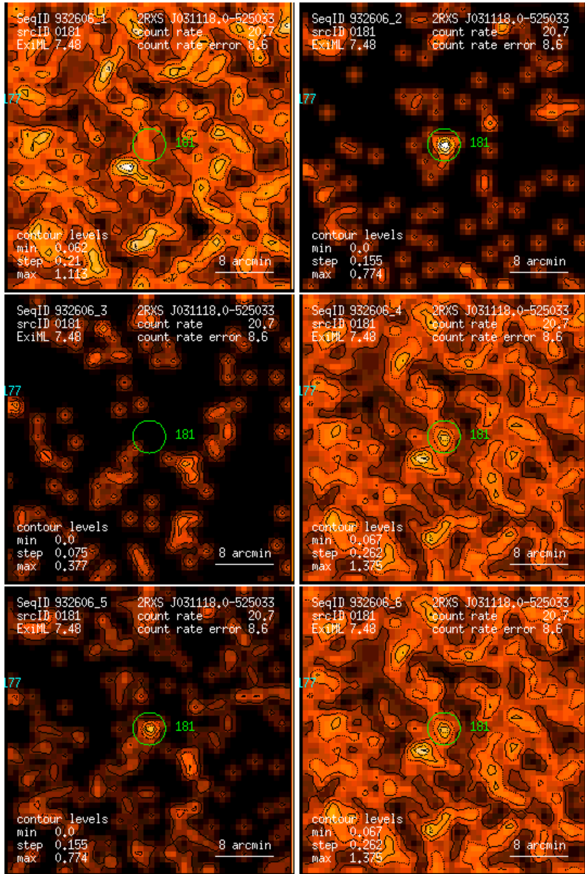
Figure 181: RASS 932606: detection 0181: band rate images, Gaussian filter: (1) PSPC channels 11 – 41, (2) 52 – 90, (3) 91 – 201, (4) 11 – 235, (5) 52 – 201, (6) 11 – 201. Broad band rates in counts/ks. Band rate contour levels in counts/ks/arcmin 2 .
