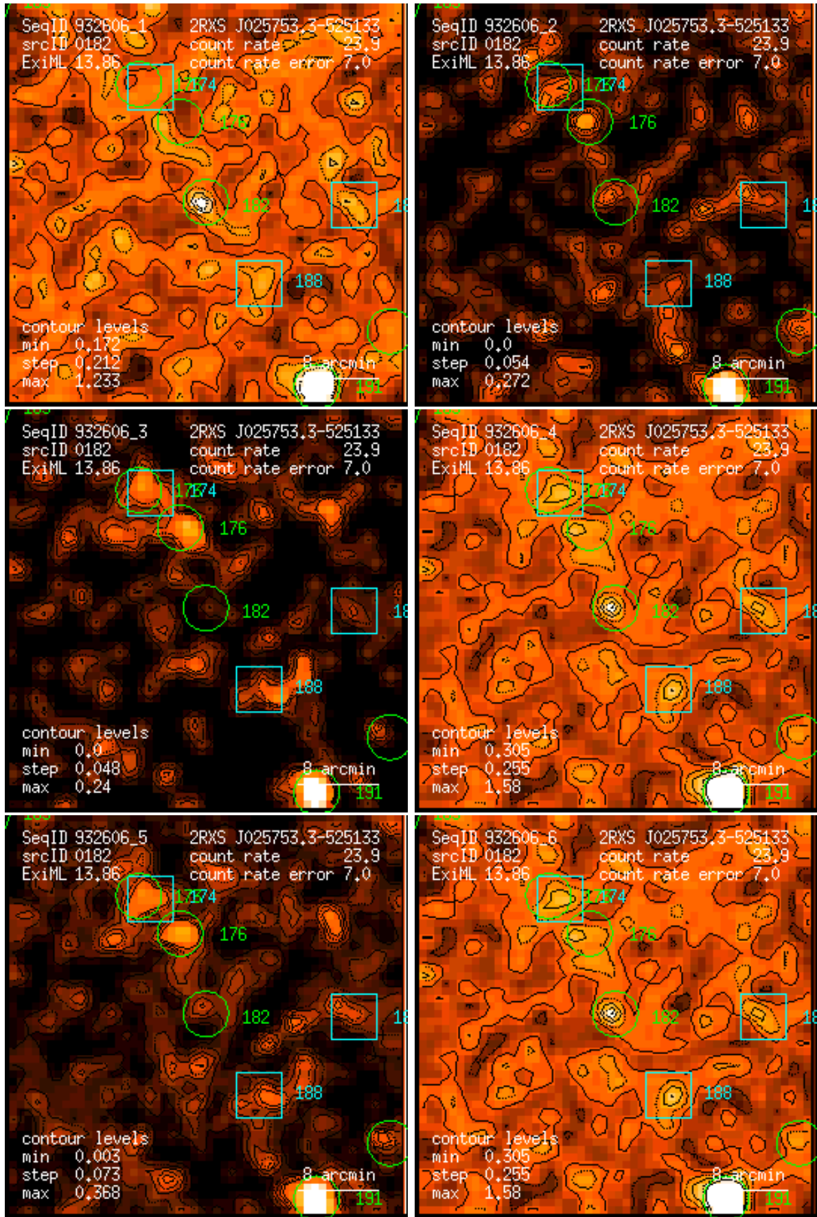
Figure 182: RASS 932606: detection 0182: band rate images, Gaussian filter: (1) PSPC channels 11 – 41, (2) 52 – 90, (3) 91 – 201, (4) 11 – 235, (5) 52 – 201, (6) 11 – 201. Broad band rates in counts/ks. Band rate contour levels in counts/ks/arcmin 2 .
