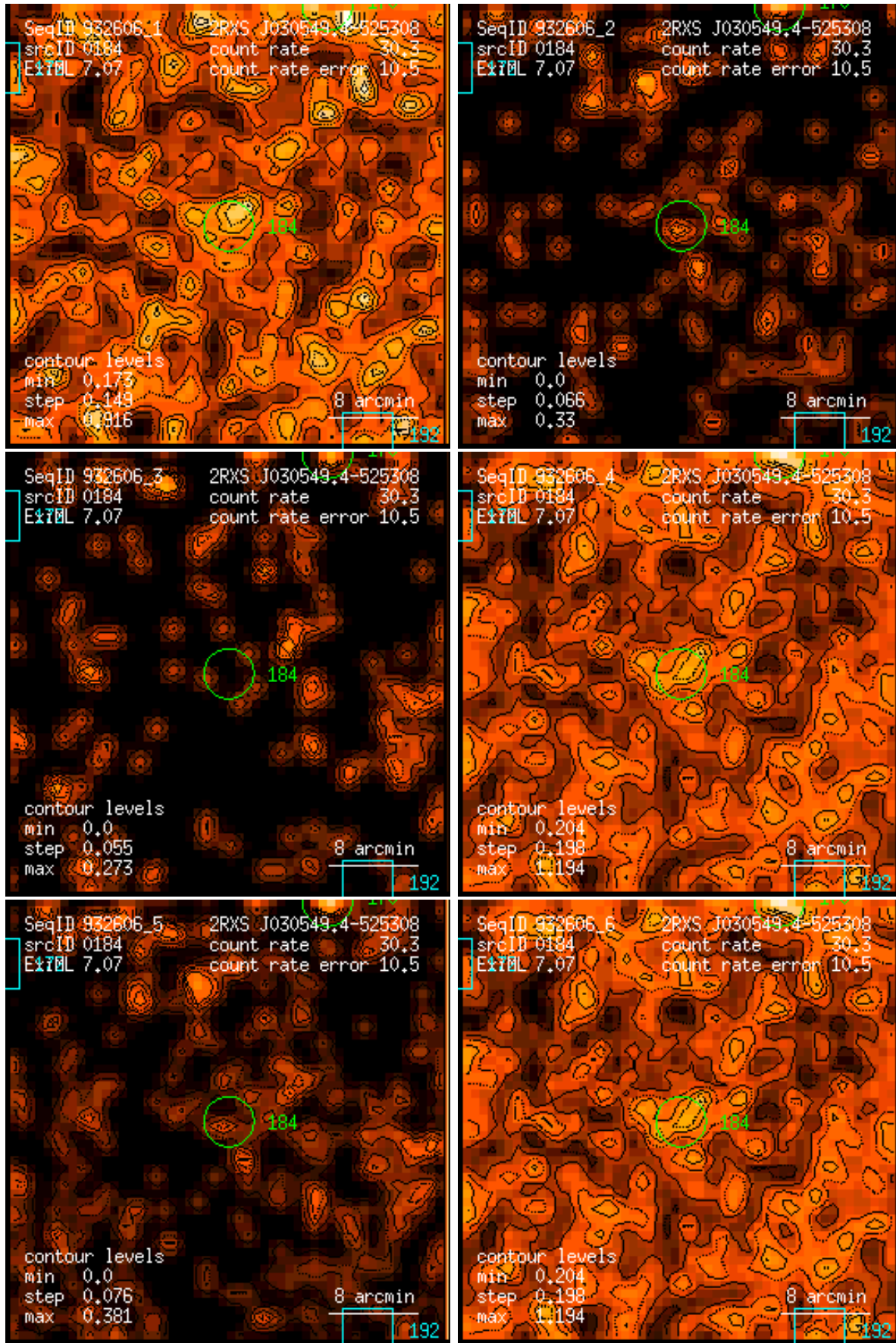
Figure 184: RASS 932606: detection 0184: band rate images, Gaussian filter: (1) PSPC channels 11 – 41, (2) 52 – 90, (3) 91 – 201, (4) 11 – 235, (5) 52 – 201, (6) 11 – 201. Broad band rates in counts/ks. Band rate contour levels in counts/ks/arcmin 2 .
