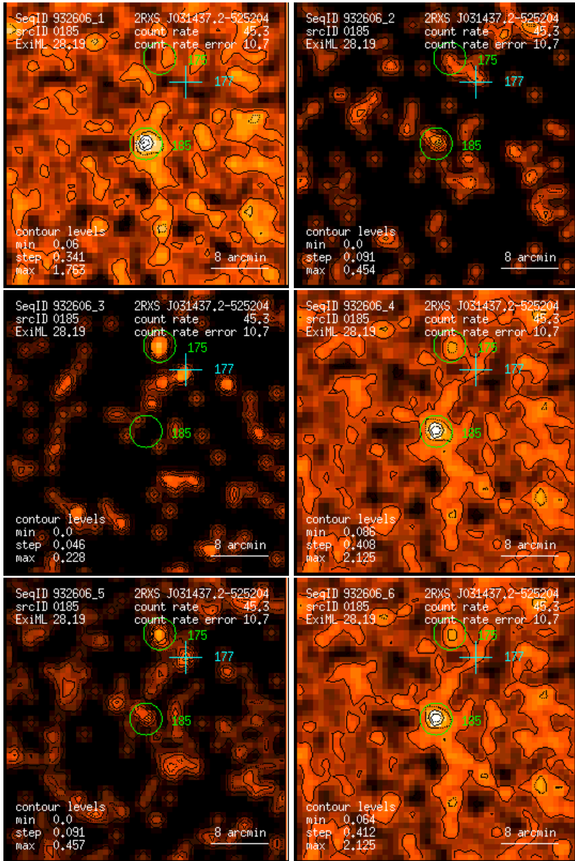
Figure 185: RASS 932606: detection 0185: band rate images, Gaussian filter: (1) PSPC channels 11 – 41, (2) 52 – 90, (3) 91 – 201, (4) 11 – 235, (5) 52 – 201, (6) 11 – 201. Broad band rates in counts/ks. Band rate contour levels in counts/ks/arcmin 2 .
