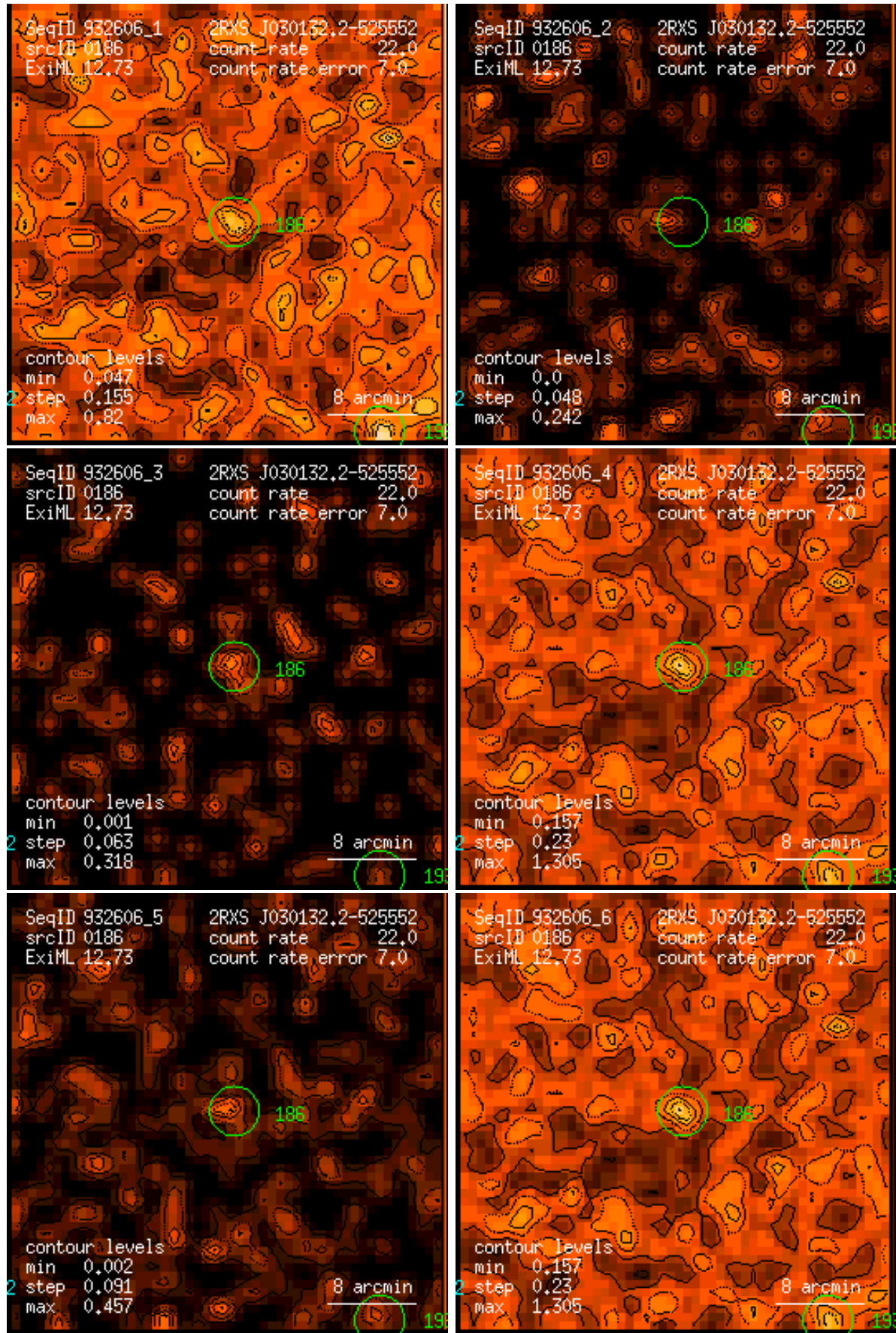
Figure 186: RASS 932606: detection 0186: band rate images, Gaussian filter: (1) PSPC channels 11 – 41, (2) 52 – 90, (3) 91 – 201, (4) 11 – 235, (5) 52 – 201, (6) 11 – 201. Broad band rates in counts/ks. Band rate contour levels in counts/ks/arcmin 2 .
