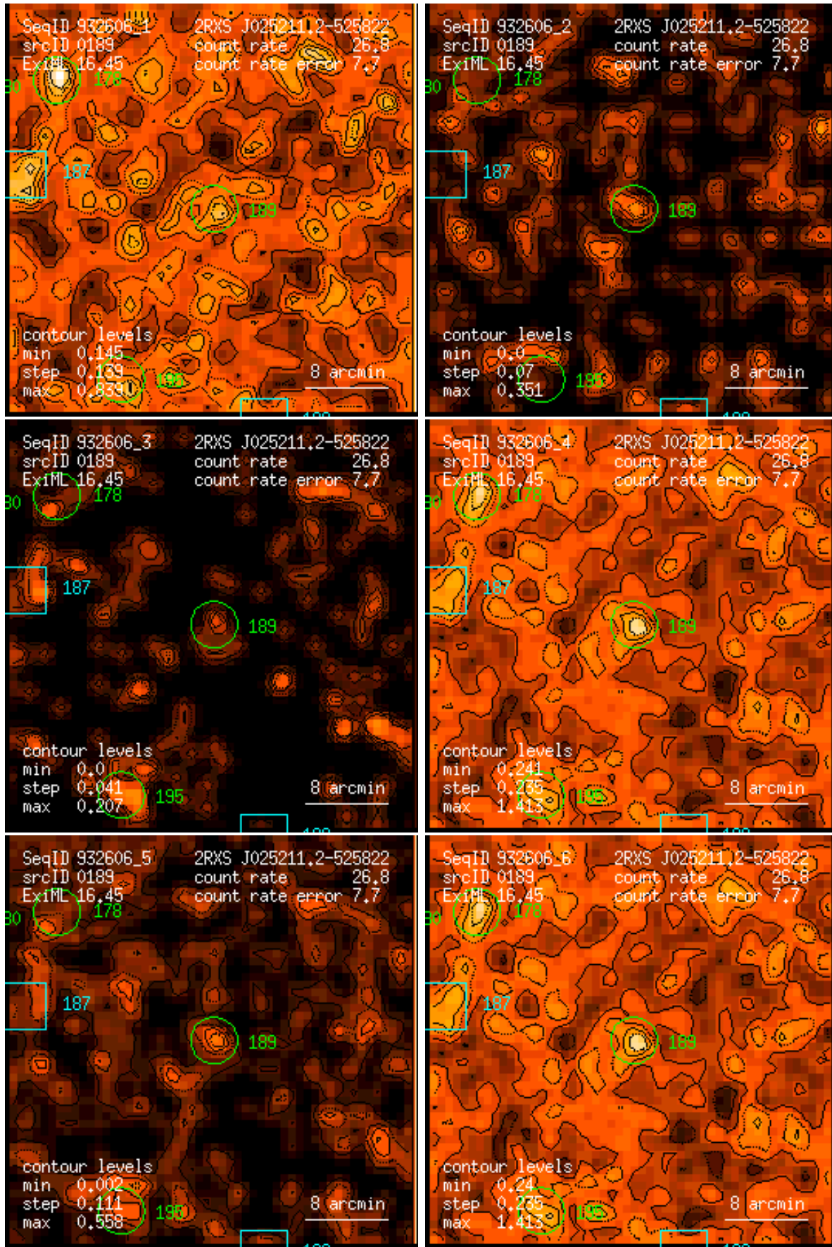
Figure 189: RASS 932606: detection 0189: band rate images, Gaussian filter: (1) PSPC channels 11 – 41, (2) 52 – 90, (3) 91 – 201, (4) 11 – 235, (5) 52 – 201, (6) 11 – 201. Broad band rates in counts/ks. Band rate contour levels in counts/ks/arcmin 2 .
