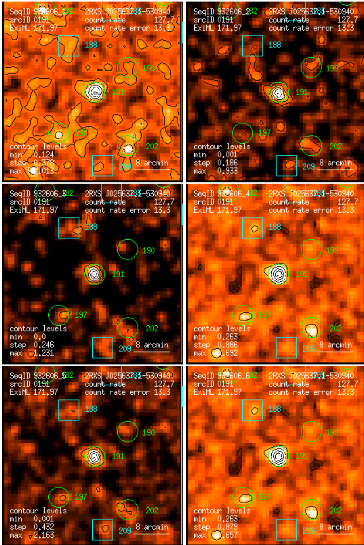
Figure 191: RASS 932606: detection 0191: band rate images, Gaussian filter: (1) PSPC channels 11 – 41, (2) 52 – 90, (3) 91 – 201, (4) 11 – 235, (5) 52 – 201, (6) 11 – 201. Broad band rates in counts/ks. Band rate contour levels in counts/ks/arcmin 2 .
