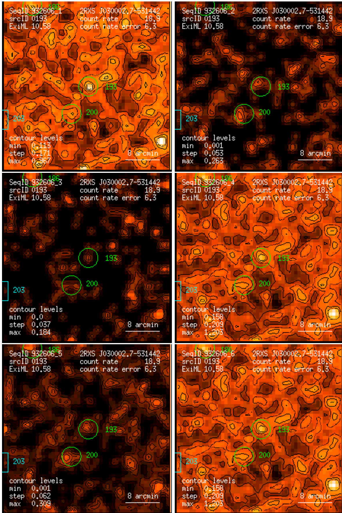
Figure 193: RASS 932606: detection 0193: band rate images, Gaussian filter: (1) PSPC channels 11 – 41, (2) 52 – 90, (3) 91 – 201, (4) 11 – 235, (5) 52 – 201, (6) 11 – 201. Broad band rates in counts/ks. Band rate contour levels in counts/ks/arcmin 2 .
