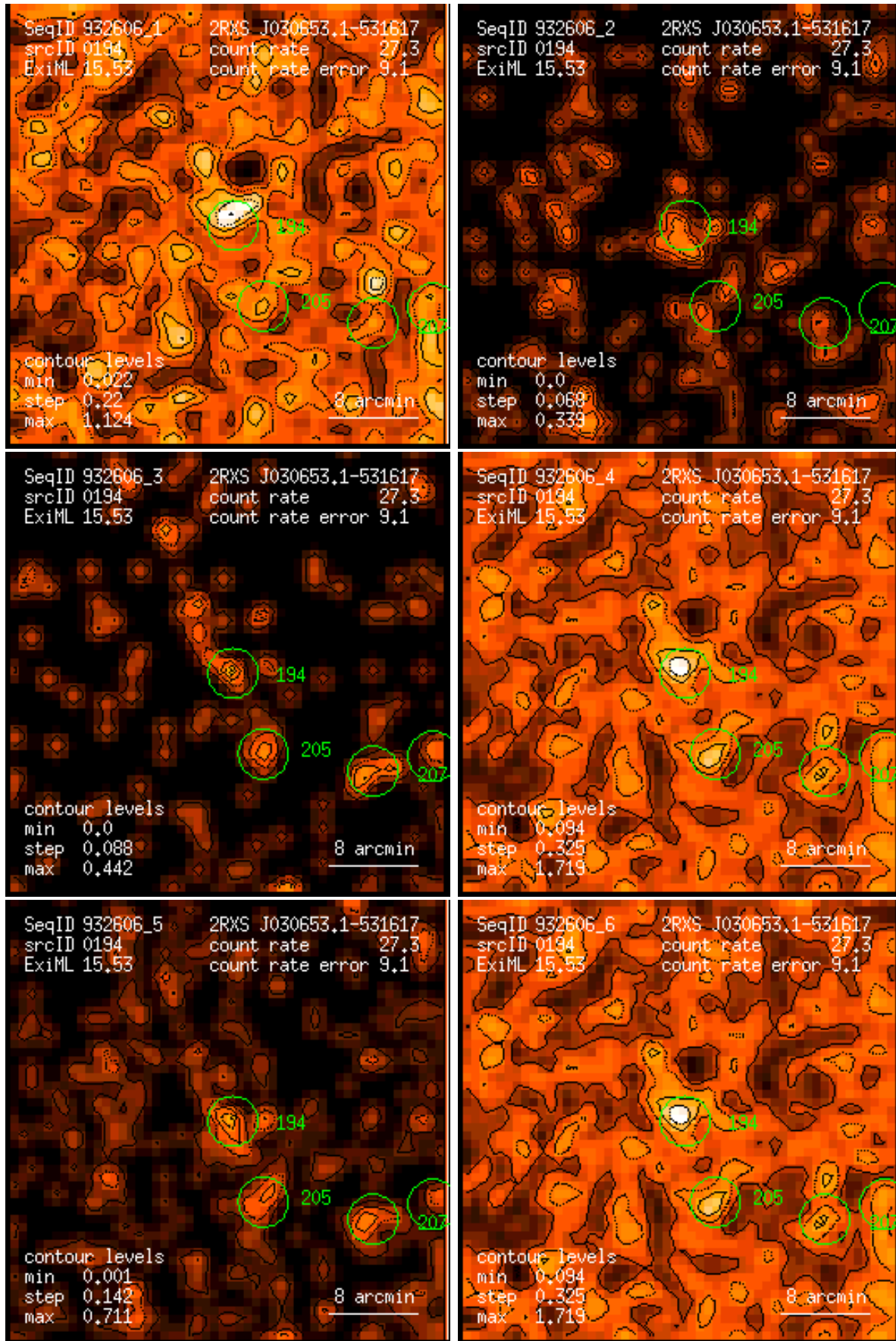
Figure 194: RASS 932606: detection 0194: band rate images, Gaussian filter: (1) PSPC channels 11 – 41, (2) 52 – 90, (3) 91 – 201, (4) 11 – 235, (5) 52 – 201, (6) 11 – 201. Broad band rates in counts/ks. Band rate contour levels in counts/ks/arcmin 2 .
