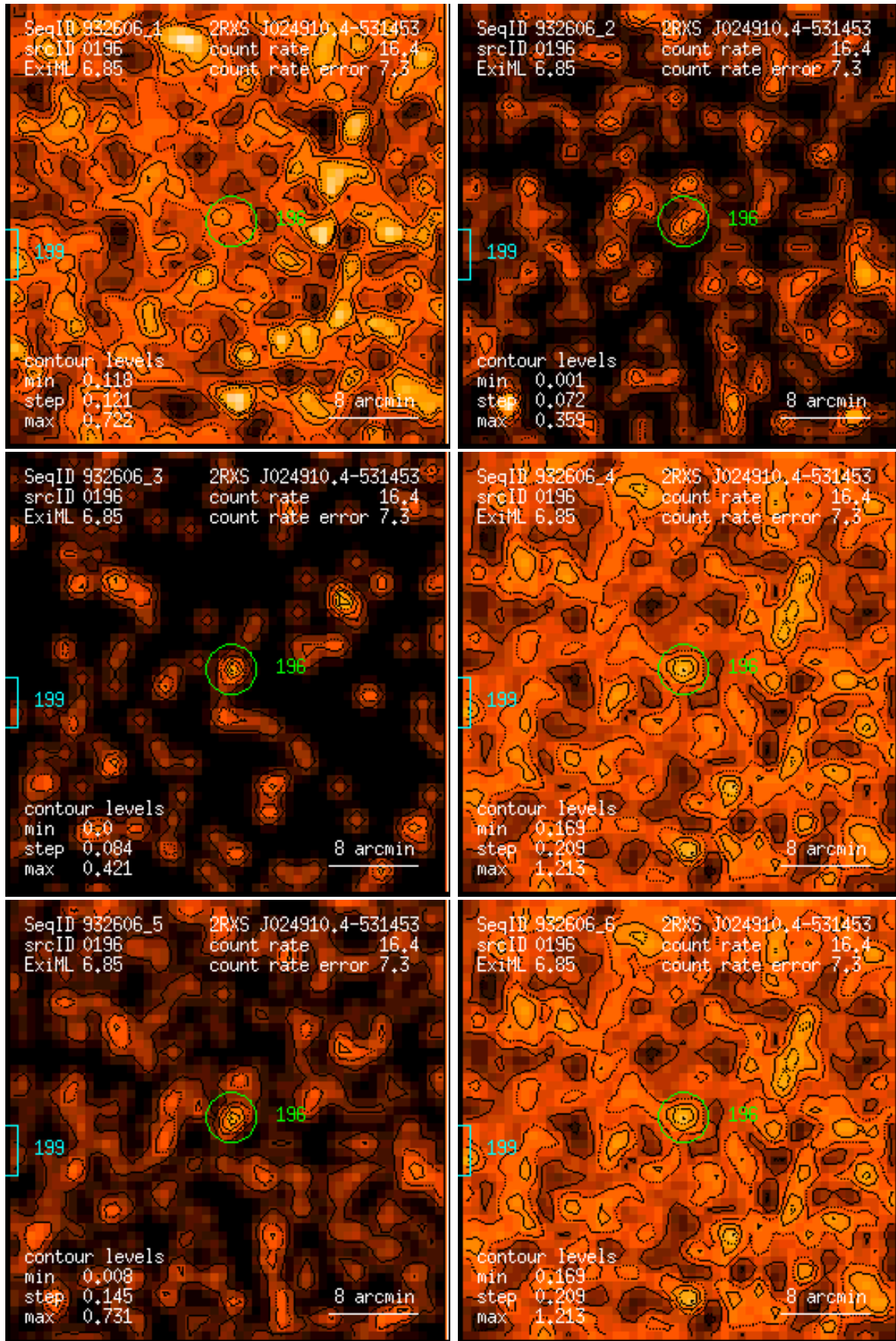
Figure 196: RASS 932606: detection 0196: band rate images, Gaussian filter: (1) PSPC channels 11 – 41, (2) 52 – 90, (3) 91 – 201, (4) 11 – 235, (5) 52 – 201, (6) 11 – 201. Broad band rates in counts/ks. Band rate contour levels in counts/ks/arcmin 2 .
