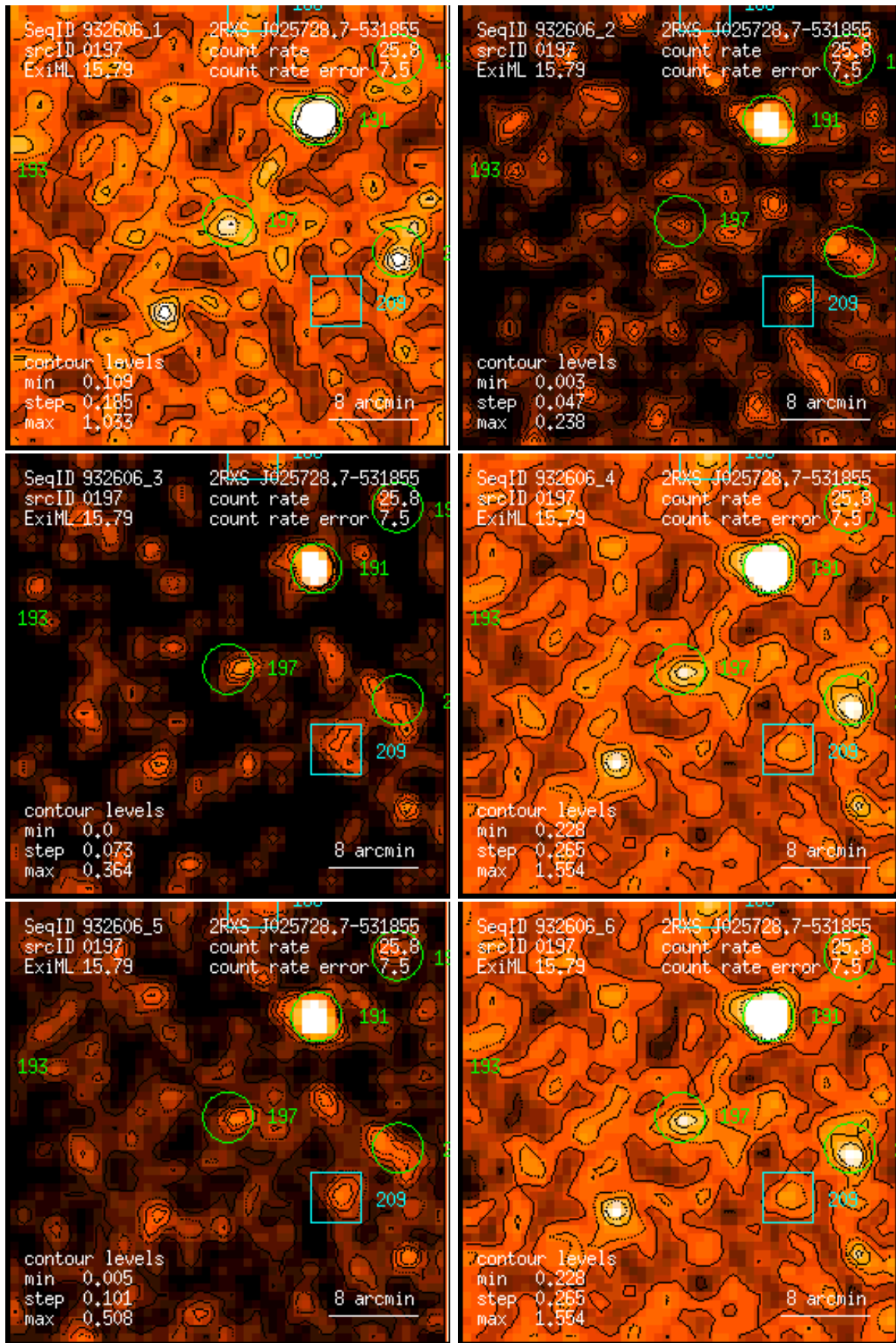
Figure 197: RASS 932606: detection 0197: band rate images, Gaussian filter: (1) PSPC channels 11 – 41, (2) 52 – 90, (3) 91 – 201, (4) 11 – 235, (5) 52 – 201, (6) 11 – 201. Broad band rates in counts/ks. Band rate contour levels in counts/ks/arcmin 2 .
