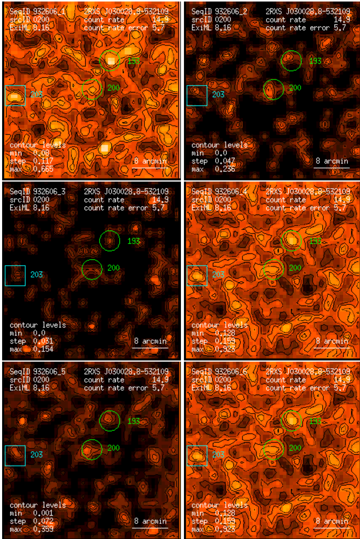
Figure 200: RASS 932606: detection 0200: band rate images, Gaussian filter: (1) PSPC channels 11 – 41, (2) 52 – 90, (3) 91 – 201, (4) 11 – 235, (5) 52 – 201, (6) 11 – 201. Broad band rates in counts/ks. Band rate contour levels in counts/ks/arcmin 2 .
