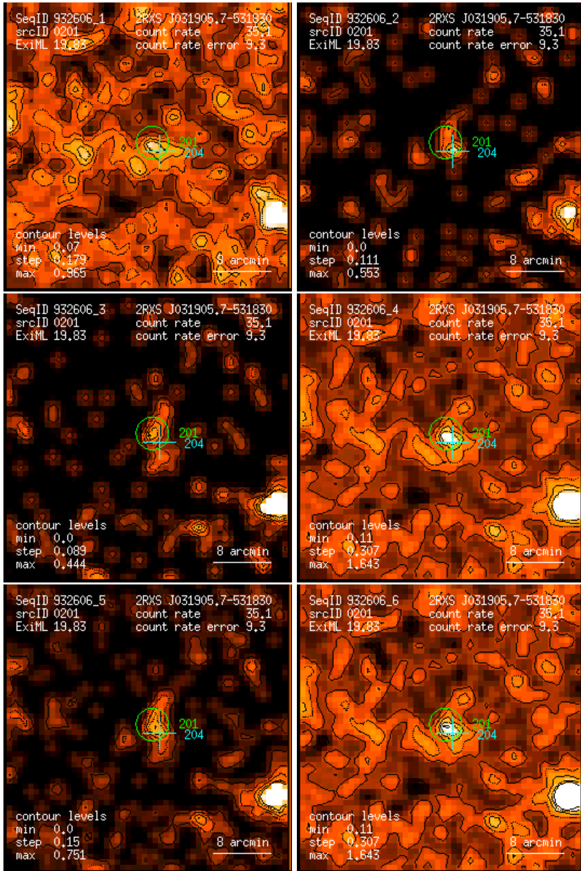
Figure 201: RASS 932606: detection 0201: band rate images, Gaussian filter: (1) PSPC channels 11 – 41, (2) 52 – 90, (3) 91 – 201, (4) 11 – 235, (5) 52 – 201, (6) 11 – 201. Broad band rates in counts/ks. Band rate contour levels in counts/ks/arcmin 2 .
