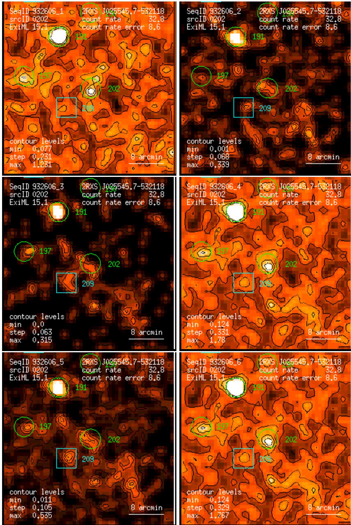
Figure 202: RASS 932606: detection 0202: band rate images, Gaussian filter: (1) PSPC channels 11 – 41, (2) 52 – 90, (3) 91 – 201, (4) 11 – 235, (5) 52 – 201, (6) 11 – 201. Broad band rates in counts/ks. Band rate contour levels in counts/ks/arcmin 2 .
