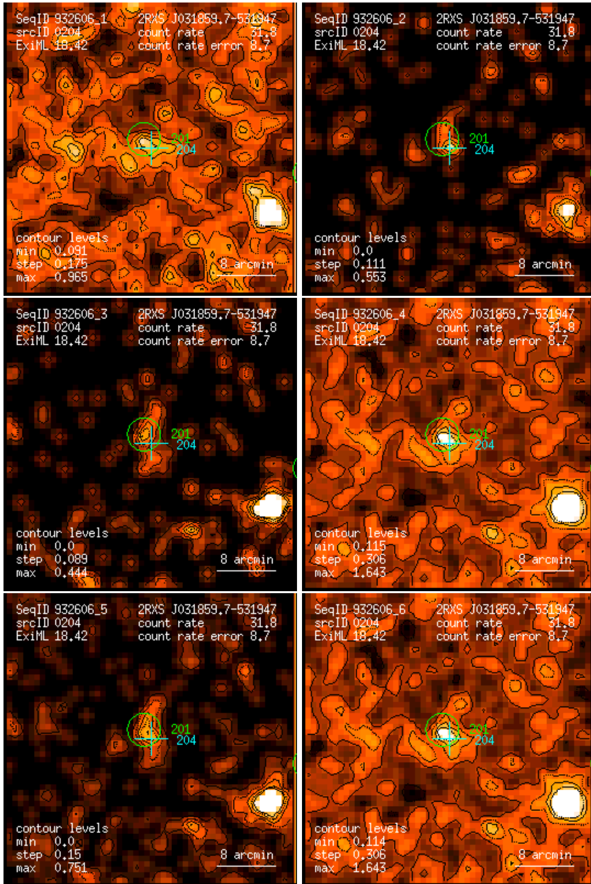
Figure 204: RASS 932606: detection 0204: band rate images, Gaussian filter: (1) PSPC channels 11 – 41, (2) 52 – 90, (3) 91 – 201, (4) 11 – 235, (5) 52 – 201, (6) 11 – 201. Broad band rates in counts/ks. Band rate contour levels in counts/ks/arcmin 2 .
