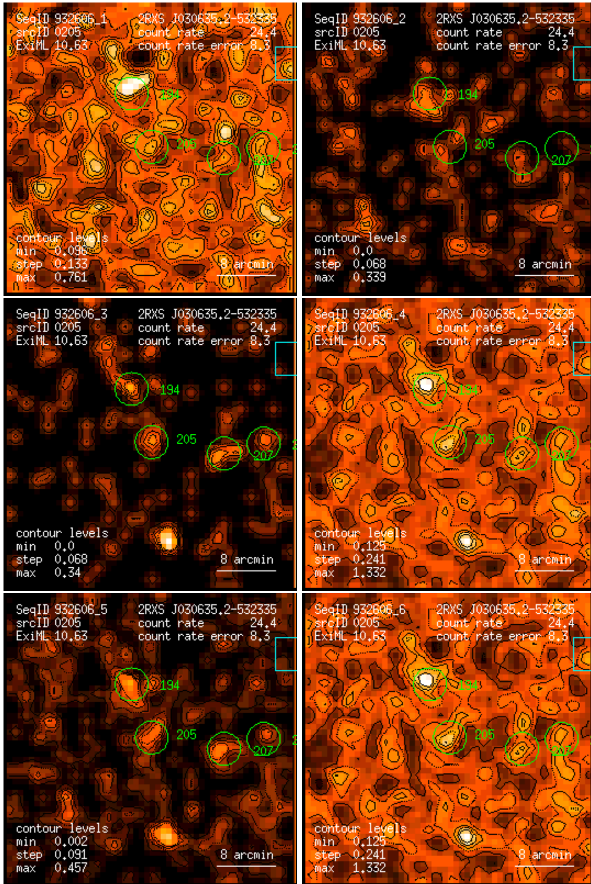
Figure 205: RASS 932606: detection 0205: band rate images, Gaussian filter: (1) PSPC channels 11 – 41, (2) 52 – 90, (3) 91 – 201, (4) 11 – 235, (5) 52 – 201, (6) 11 – 201. Broad band rates in counts/ks. Band rate contour levels in counts/ks/arcmin 2 .
