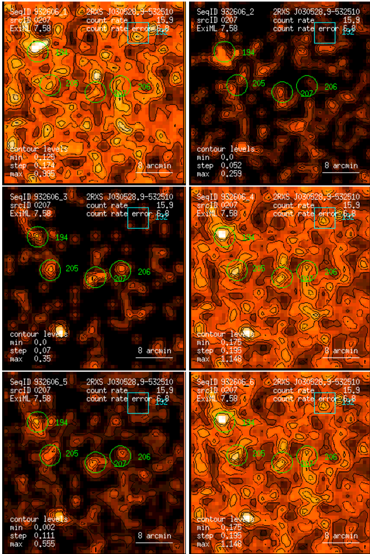
Figure 207: RASS 932606: detection 0207: band rate images, Gaussian filter: (1) PSPC channels 11 – 41, (2) 52 – 90, (3) 91 – 201, (4) 11 – 235, (5) 52 – 201, (6) 11 – 201. Broad band rates in counts/ks. Band rate contour levels in counts/ks/arcmin 2 .
