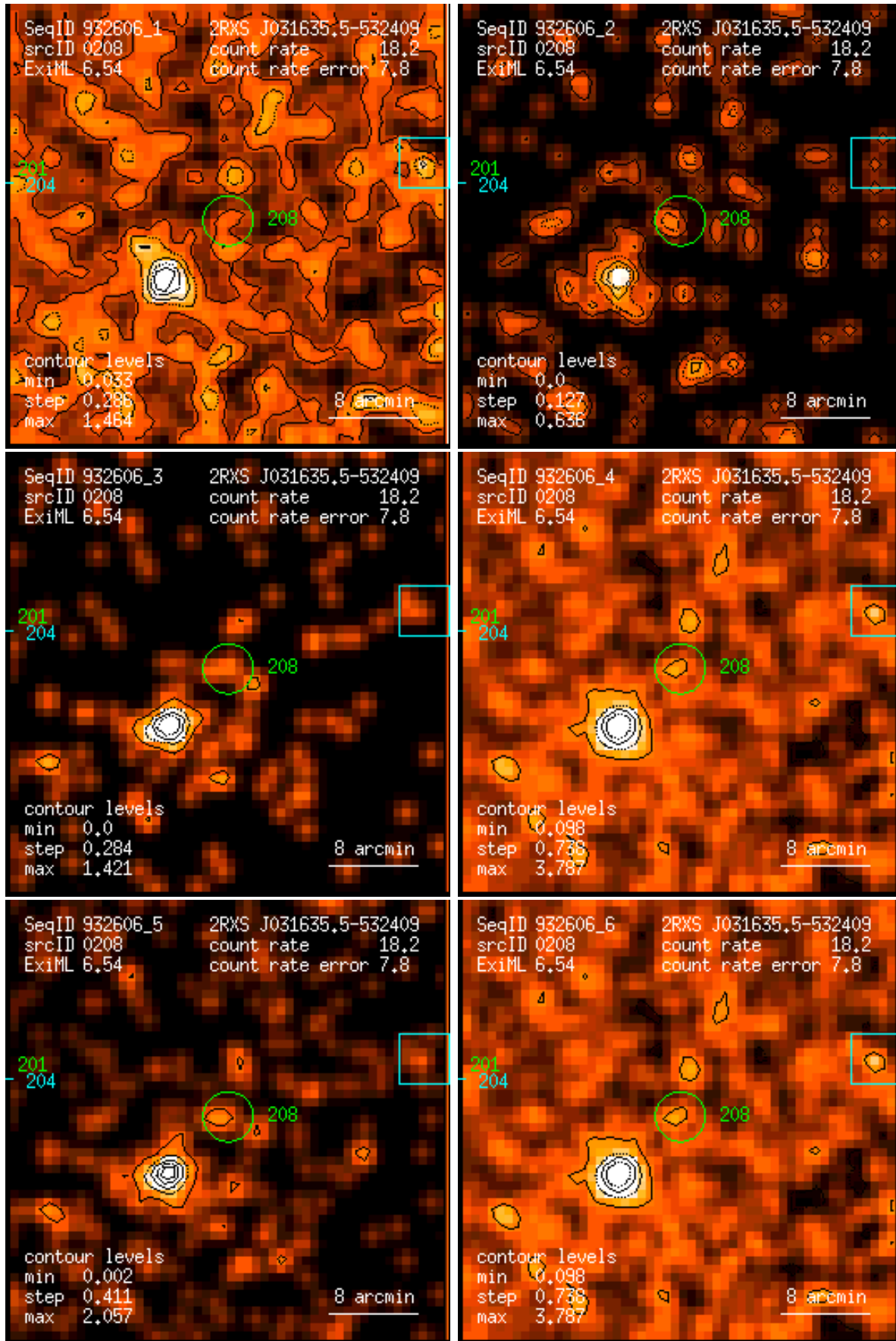
Figure 208: RASS 932606: detection 0208: band rate images, Gaussian filter: (1) PSPC channels 11 – 41, (2) 52 – 90, (3) 91 – 201, (4) 11 – 235, (5) 52 – 201, (6) 11 – 201. Broad band rates in counts/ks. Band rate contour levels in counts/ks/arcmin 2 .
