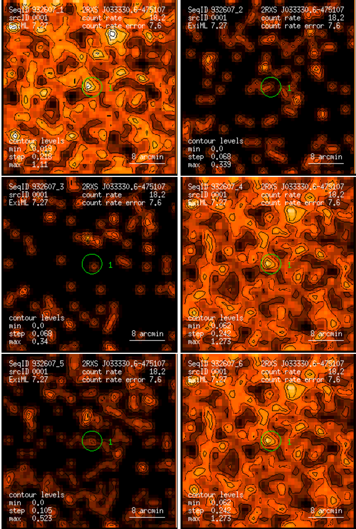
Figure 1: RASS 932607: detection 0001: band rate images, Gaussian filter: (1) PSPC channels 11 – 41, (2) 52 – 90, (3) 91 – 201, (4) 11 – 235, (5) 52 – 201, (6) 11 – 201. Broad band rates in counts/ks. Band rate contour levels in counts/ks/arcmin 2 .
