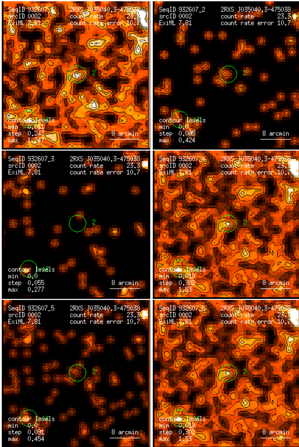
Figure 2: RASS 932607: detection 0002: band rate images, Gaussian filter: (1) PSPC channels 11 – 41, (2) 52 – 90, (3) 91 – 201, (4) 11 – 235, (5) 52 – 201, (6) 11 – 201. Broad band rates in counts/ks. Band rate contour levels in counts/ks/arcmin 2 .
