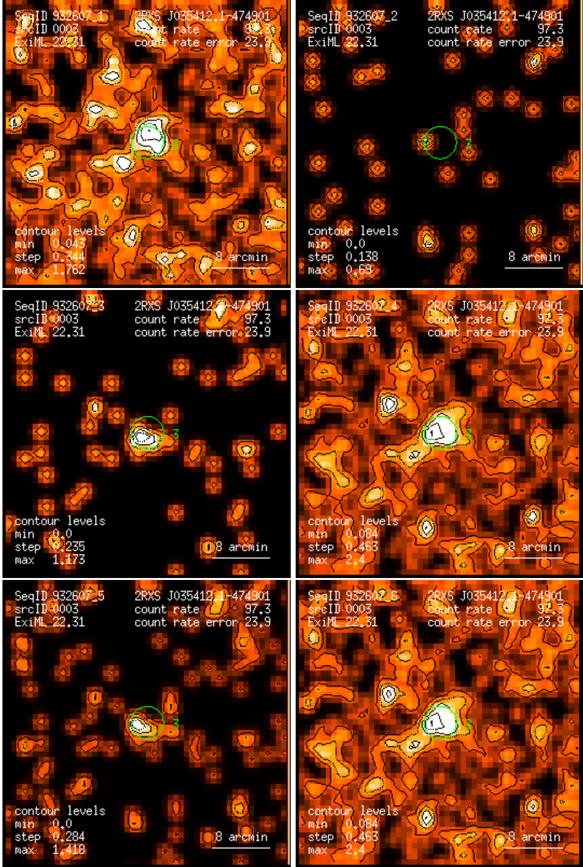
Figure 3: RASS 932607: detection 0003: band rate images, Gaussian filter: (1) PSPC channels 11 – 41, (2) 52 – 90, (3) 91 – 201, (4) 11 – 235, (5) 52 – 201, (6) 11 – 201. Broad band rates in counts/ks. Band rate contour levels in counts/ks/arcmin 2 .
