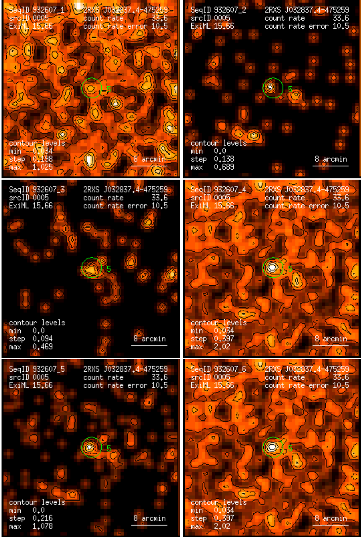
Figure 5: RASS 932607: detection 0005: band rate images, Gaussian filter: (1) PSPC channels 11 – 41, (2) 52 – 90, (3) 91 – 201, (4) 11 – 235, (5) 52 – 201, (6) 11 – 201. Broad band rates in counts/ks. Band rate contour levels in counts/ks/arcmin 2 .
