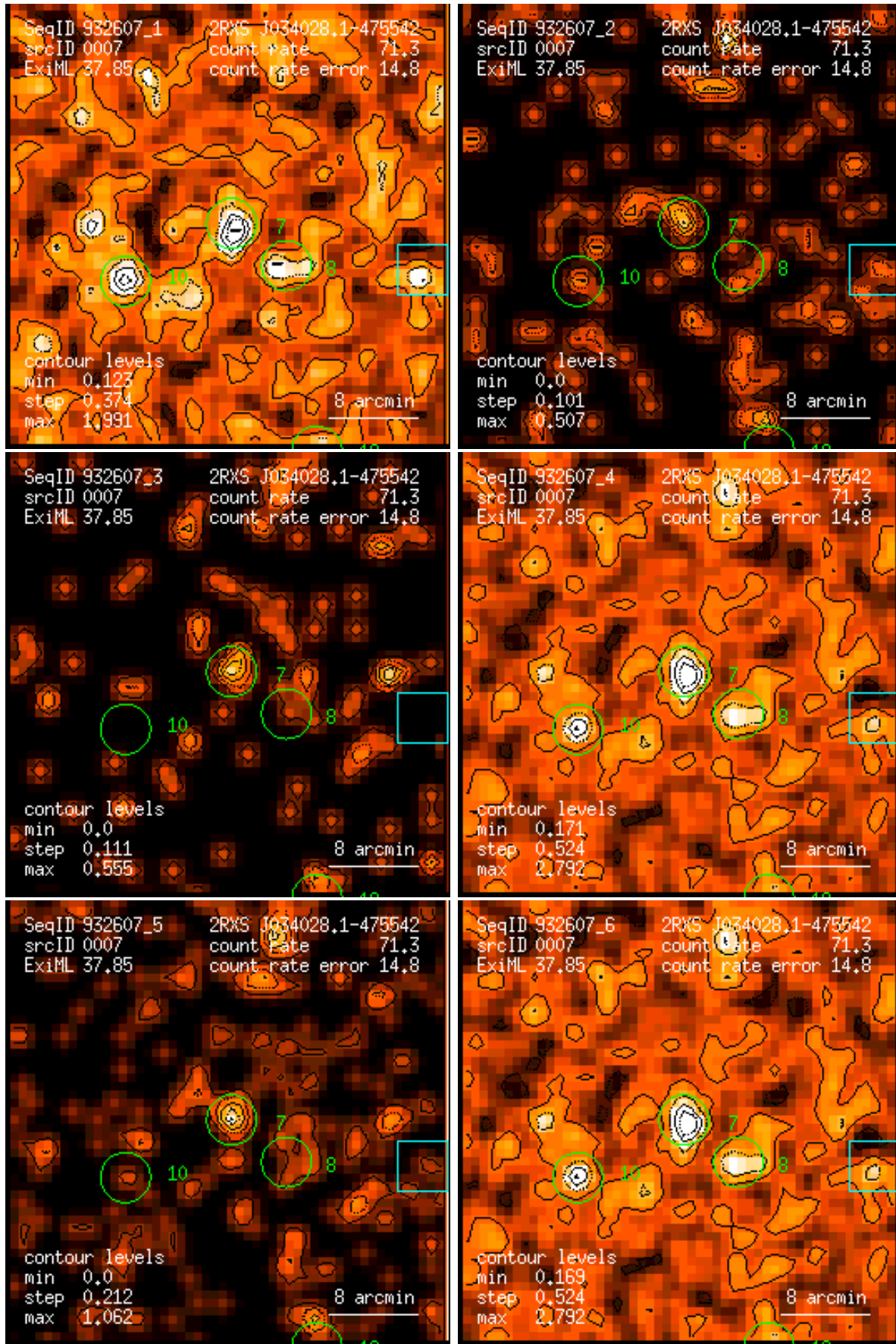
Figure 7: RASS 932607: detection 0007: band rate images, Gaussian filter: (1) PSPC channels 11 – 41, (2) 52 – 90, (3) 91 – 201, (4) 11 – 235, (5) 52 – 201, (6) 11 – 201. Broad band rates in counts/ks. Band rate contour levels in counts/ks/arcmin 2 .
