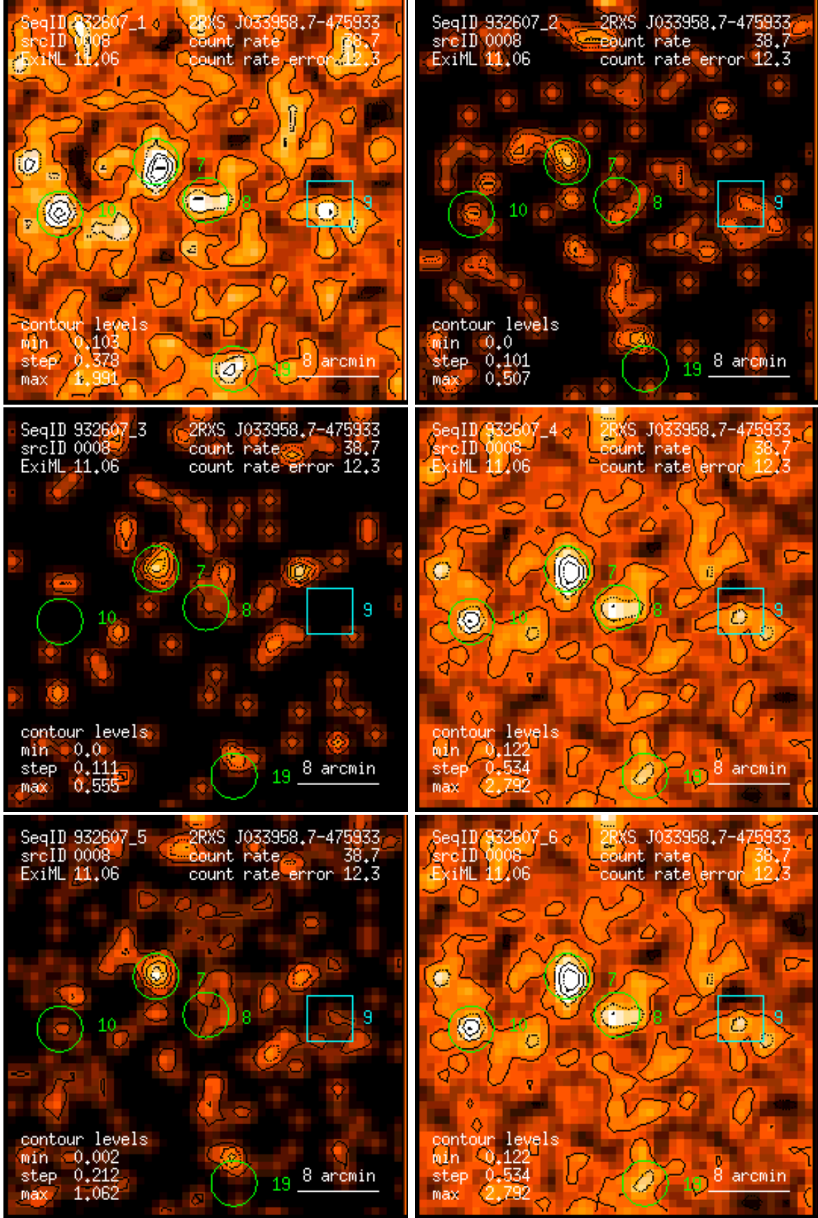
Figure 8: RASS 932607: detection 0008: band rate images, Gaussian filter: (1) PSPC channels 11 – 41, (2) 52 – 90, (3) 91 – 201, (4) 11 – 235, (5) 52 – 201, (6) 11 – 201. Broad band rates in counts/ks. Band rate contour levels in counts/ks/arcmin 2 .
