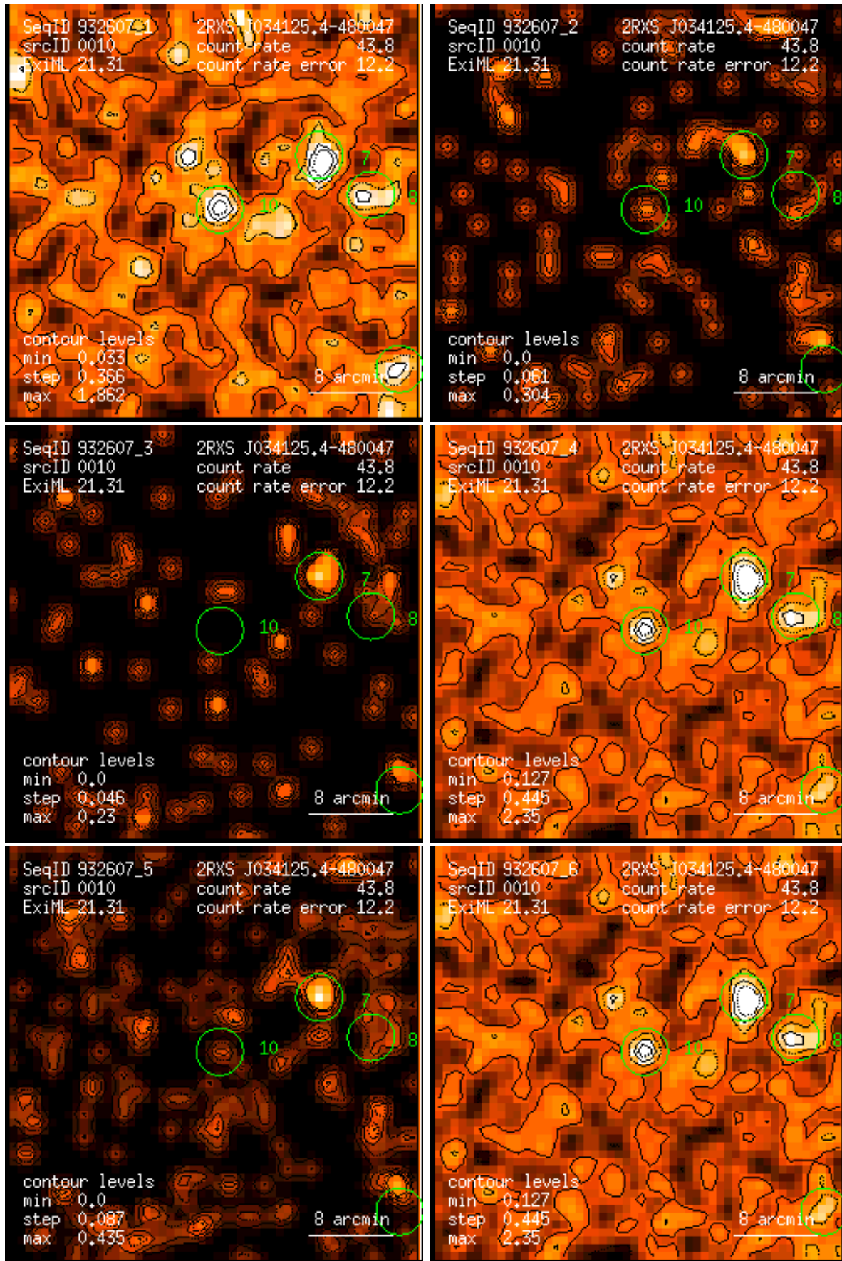
Figure 10: RASS 932607: detection 0010: band rate images, Gaussian filter: (1) PSPC channels 11 – 41, (2) 52 – 90, (3) 91 – 201, (4) 11 – 235, (5) 52 – 201, (6) 11 – 201. Broad band rates in counts/ks. Band rate contour levels in counts/ks/arcmin 2 .
