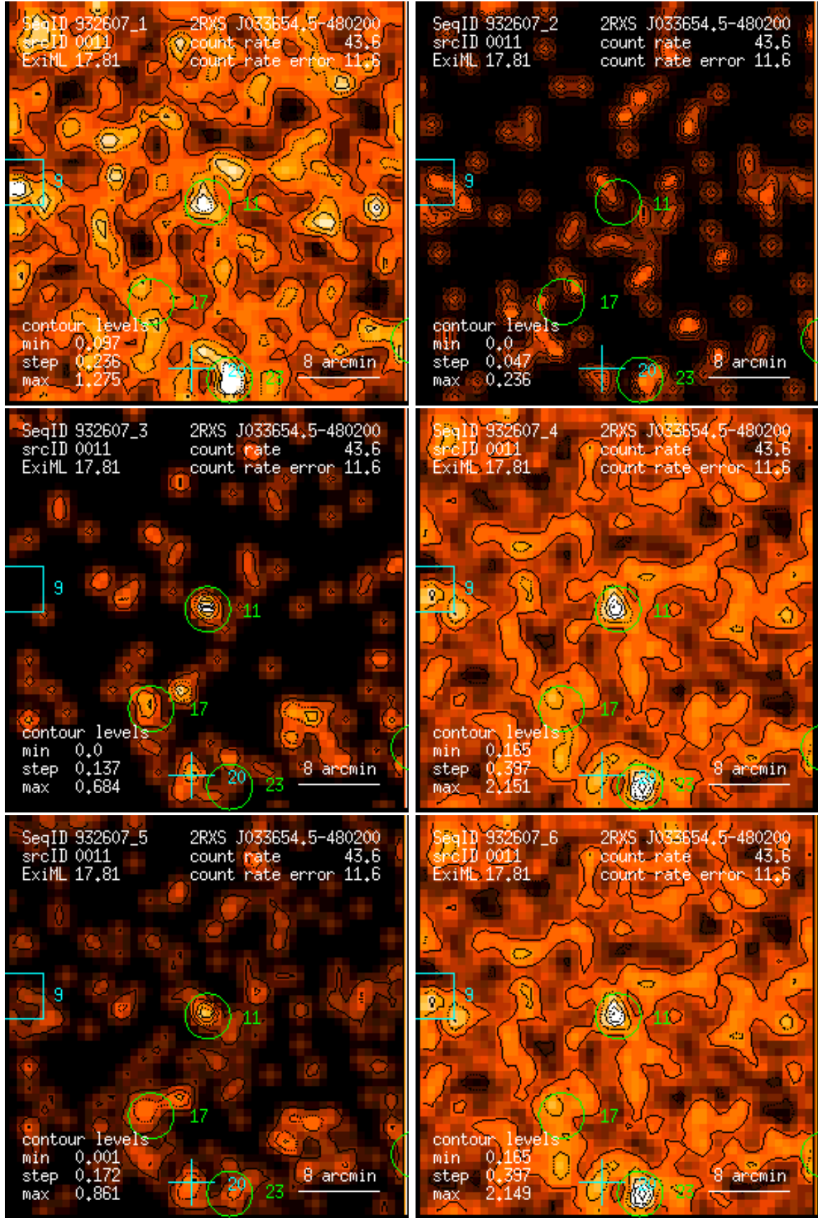
Figure 11: RASS 932607: detection 0011: band rate images, Gaussian filter: (1) PSPC channels 11 – 41, (2) 52 – 90, (3) 91 – 201, (4) 11 – 235, (5) 52 – 201, (6) 11 – 201. Broad band rates in counts/ks. Band rate contour levels in counts/ks/arcmin 2 .
