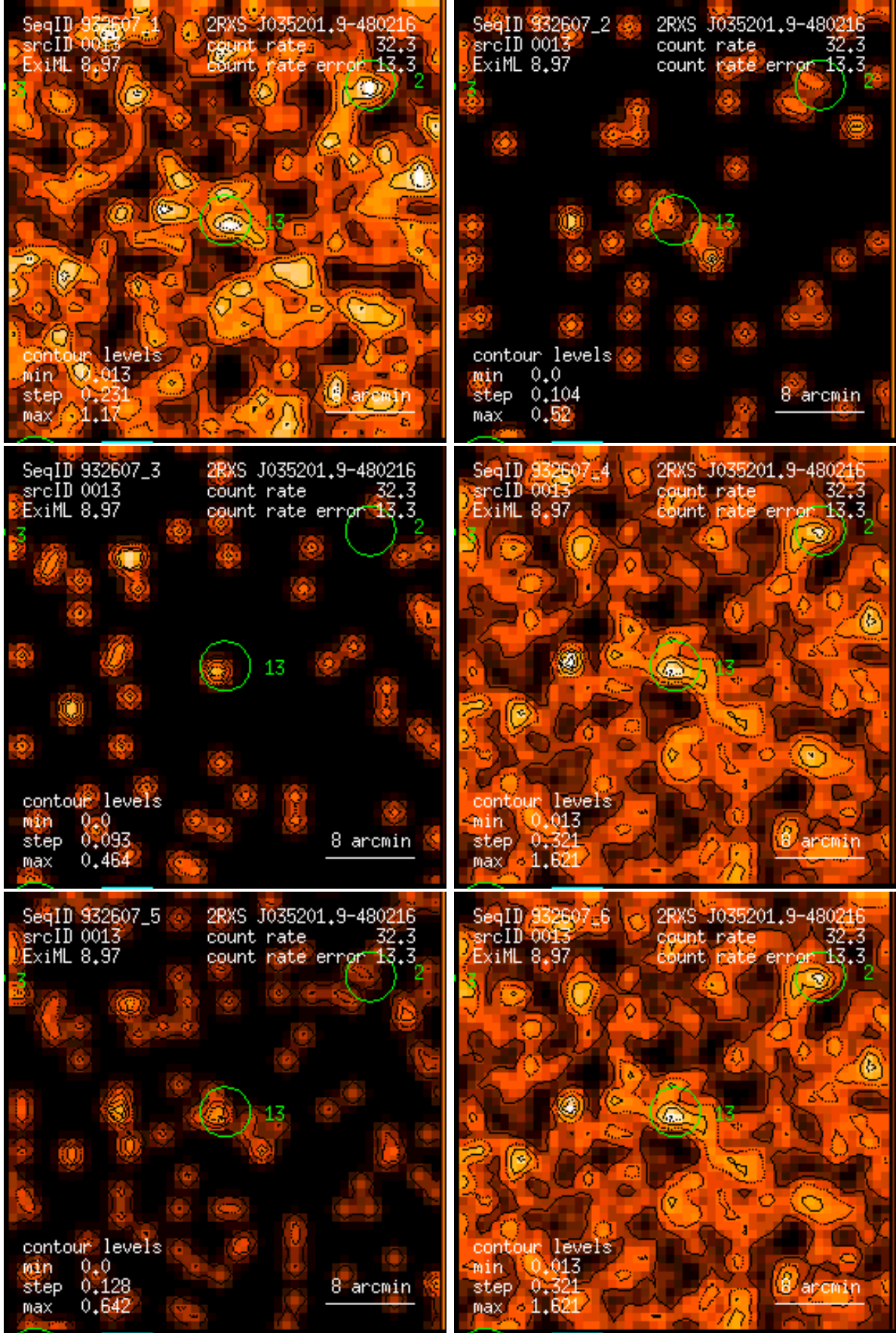
Figure 13: RASS 932607: detection 0013: band rate images, Gaussian filter: (1) PSPC channels 11 – 41, (2) 52 – 90, (3) 91 – 201, (4) 11 – 235, (5) 52 – 201, (6) 11 – 201. Broad band rates in counts/ks. Band rate contour levels in counts/ks/arcmin 2 .
