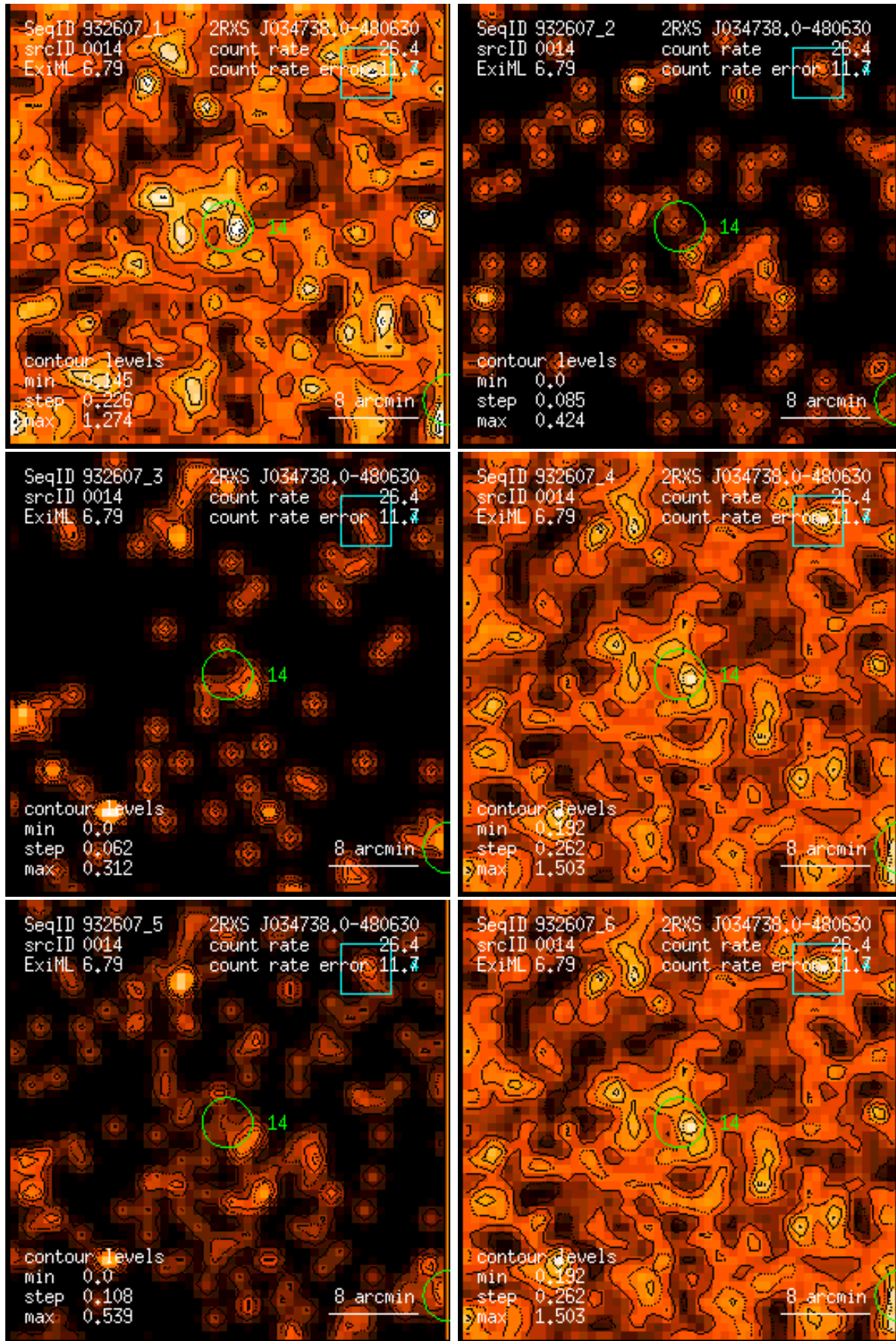
Figure 14: RASS 932607: detection 0014: band rate images, Gaussian filter: (1) PSPC channels 11 – 41, (2) 52 – 90, (3) 91 – 201, (4) 11 – 235, (5) 52 – 201, (6) 11 – 201. Broad band rates in counts/ks. Band rate contour levels in counts/ks/arcmin 2 .
