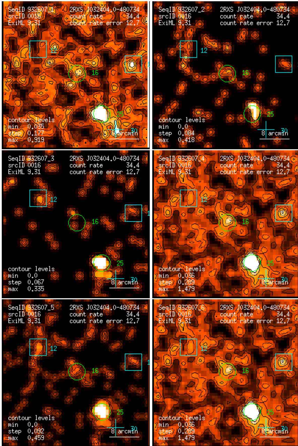
Figure 16: RASS 932607: detection 0016: band rate images, Gaussian filter: (1) PSPC channels 11 – 41, (2) 52 – 90, (3) 91 – 201, (4) 11 – 235, (5) 52 – 201, (6) 11 – 201. Broad band rates in counts/ks. Band rate contour levels in counts/ks/arcmin 2 .
