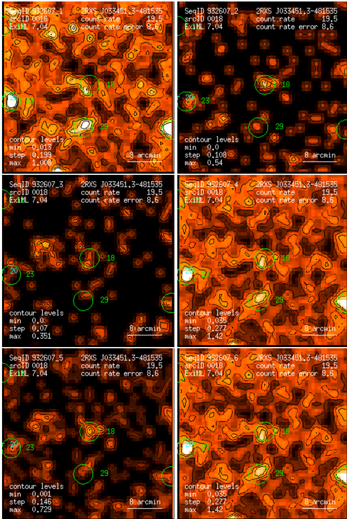
Figure 18: RASS 932607: detection 0018: band rate images, Gaussian filter: (1) PSPC channels 11 – 41, (2) 52 – 90, (3) 91 – 201, (4) 11 – 235, (5) 52 – 201, (6) 11 – 201. Broad band rates in counts/ks. Band rate contour levels in counts/ks/arcmin 2 .
