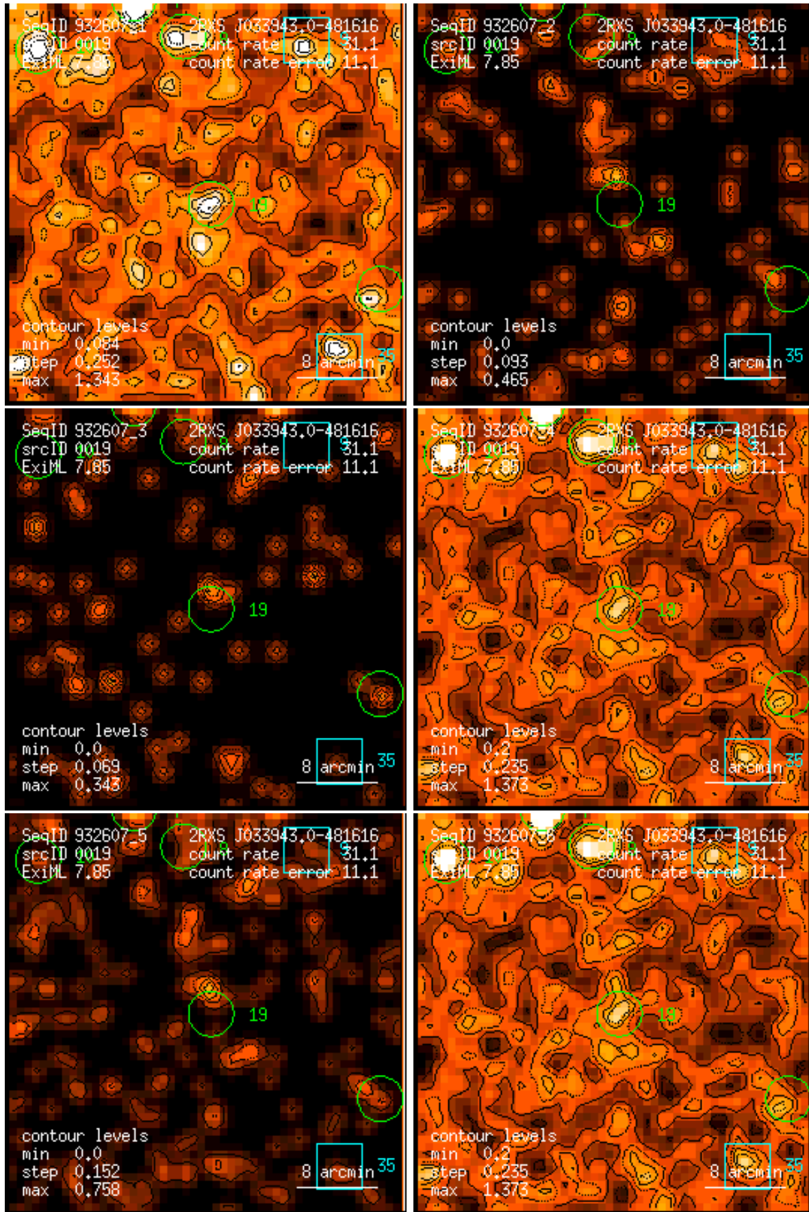
Figure 19: RASS 932607: detection 0019: band rate images, Gaussian filter: (1) PSPC channels 11 – 41, (2) 52 – 90, (3) 91 – 201, (4) 11 – 235, (5) 52 – 201, (6) 11 – 201. Broad band rates in counts/ks. Band rate contour levels in counts/ks/arcmin 2 .
