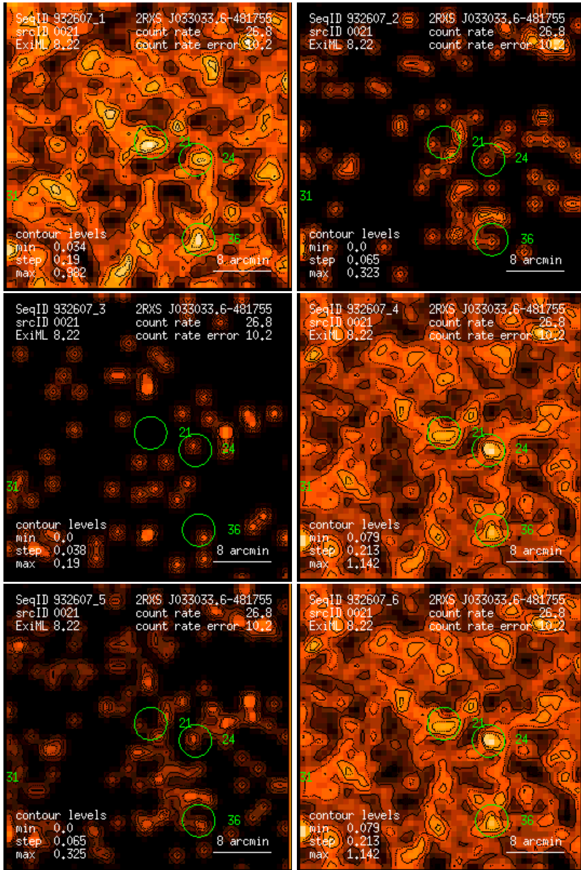
Figure 21: RASS 932607: detection 0021: band rate images, Gaussian filter: (1) PSPC channels 11 – 41, (2) 52 – 90, (3) 91 – 201, (4) 11 – 235, (5) 52 – 201, (6) 11 – 201. Broad band rates in counts/ks. Band rate contour levels in counts/ks/arcmin 2 .
