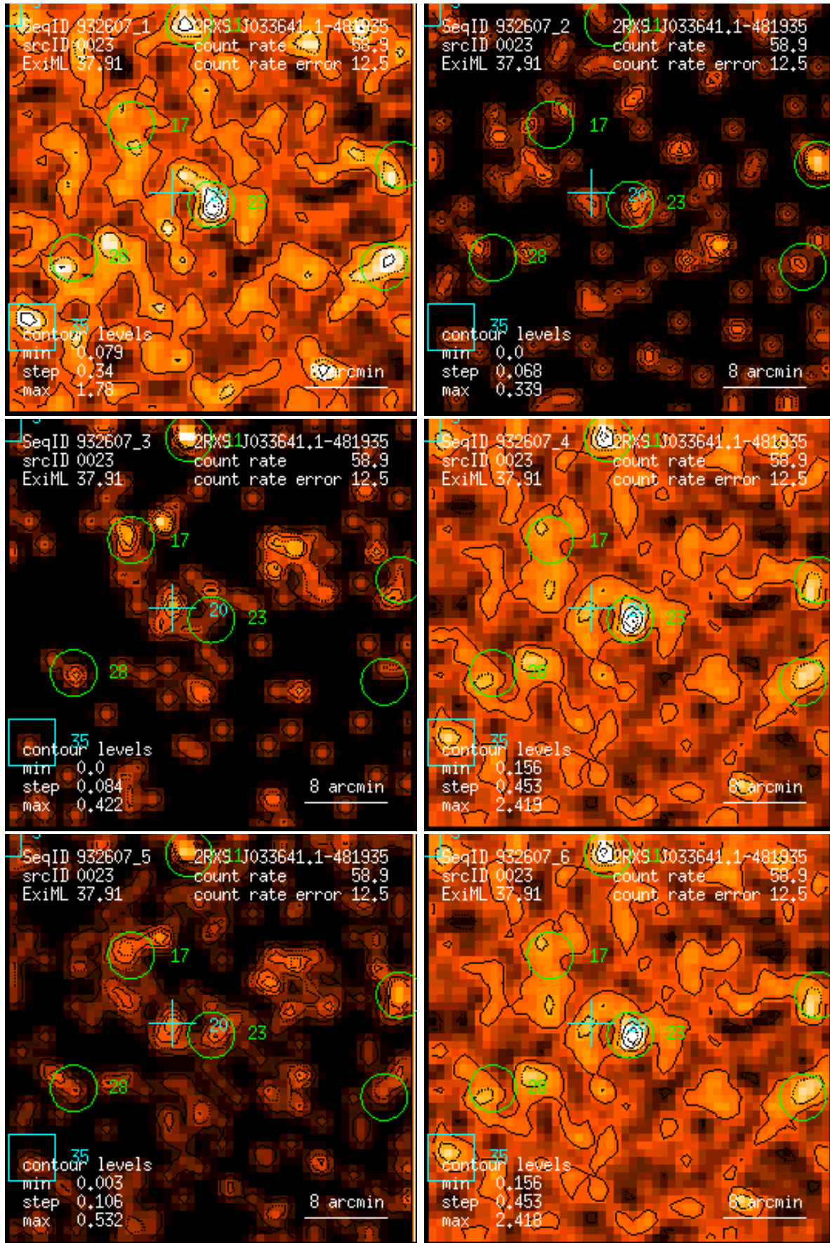
Figure 23: RASS 932607: detection 0023: band rate images, Gaussian filter: (1) PSPC channels 11 – 41, (2) 52 – 90, (3) 91 – 201, (4) 11 – 235, (5) 52 – 201, (6) 11 – 201. Broad band rates in counts/ks. Band rate contour levels in counts/ks/arcmin 2 .
