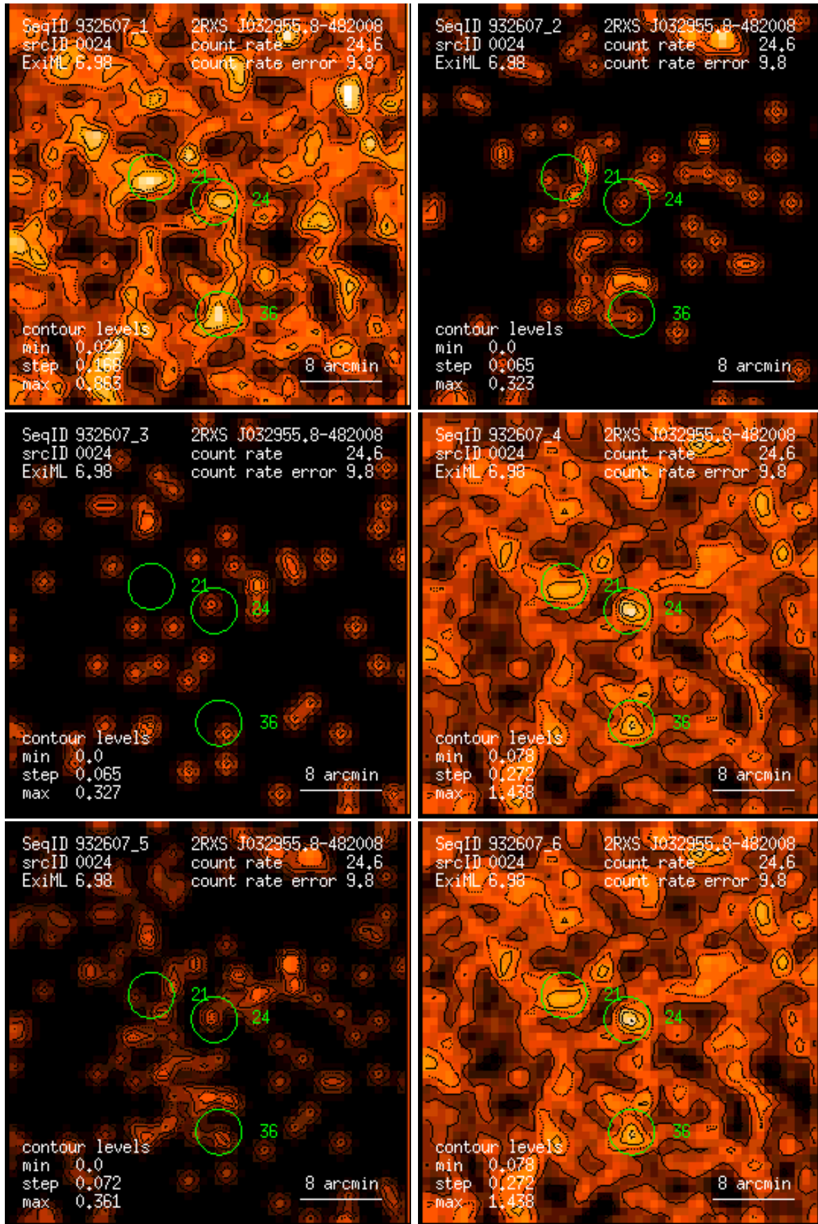
Figure 24: RASS 932607: detection 0024: band rate images, Gaussian filter: (1) PSPC channels 11 – 41, (2) 52 – 90, (3) 91 – 201, (4) 11 – 235, (5) 52 – 201, (6) 11 – 201. Broad band rates in counts/ks. Band rate contour levels in counts/ks/arcmin 2 .
