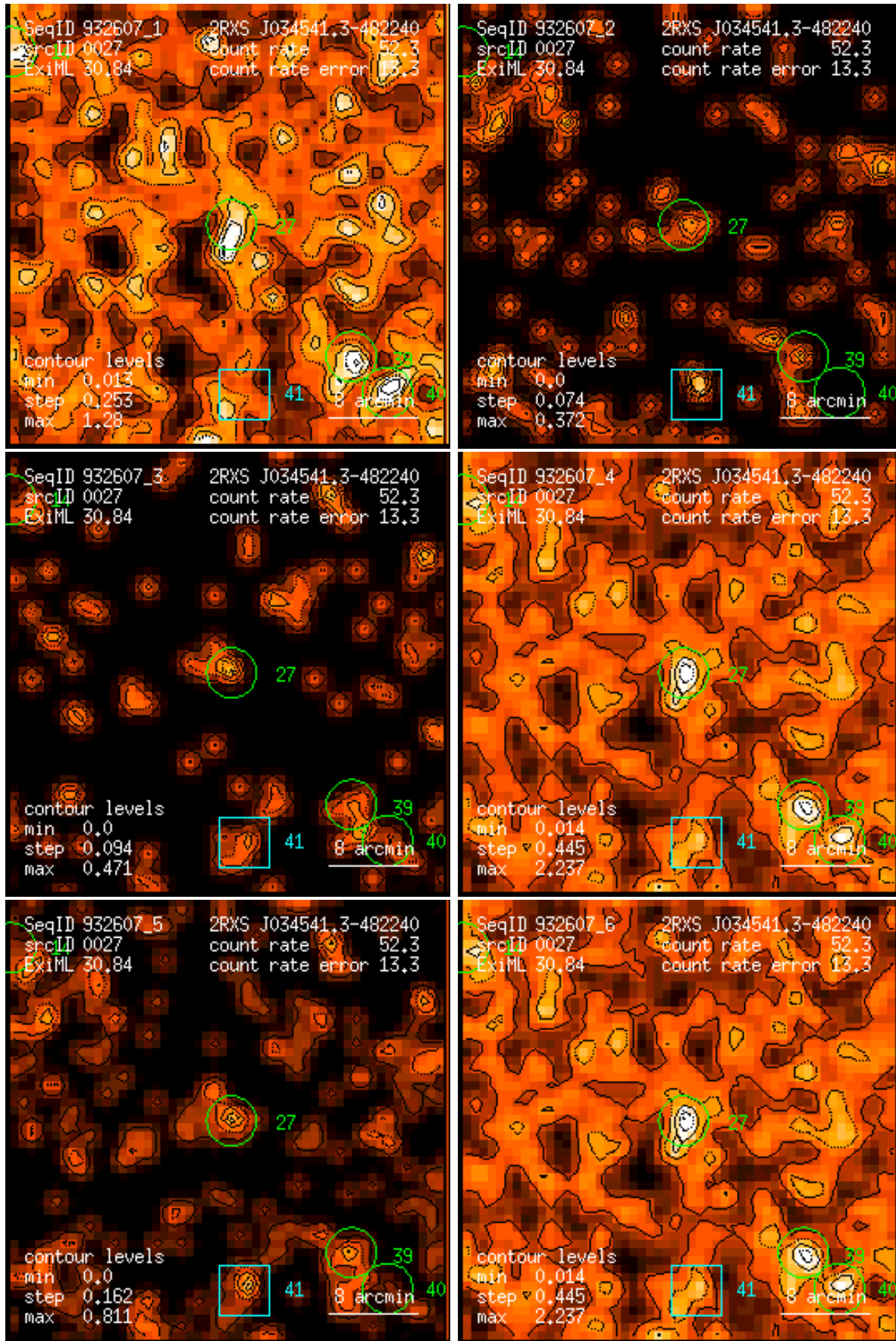
Figure 27: RASS 932607: detection 0027: band rate images, Gaussian filter: (1) PSPC channels 11 – 41, (2) 52 – 90, (3) 91 – 201, (4) 11 – 235, (5) 52 – 201, (6) 11 – 201. Broad band rates in counts/ks. Band rate contour levels in counts/ks/arcmin 2 .
