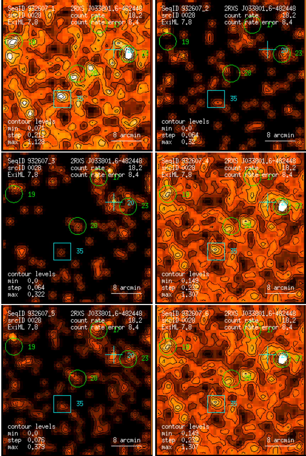
Figure 28: RASS 932607: detection 0028: band rate images, Gaussian filter: (1) PSPC channels 11 – 41, (2) 52 – 90, (3) 91 – 201, (4) 11 – 235, (5) 52 – 201, (6) 11 – 201. Broad band rates in counts/ks. Band rate contour levels in counts/ks/arcmin 2 .
