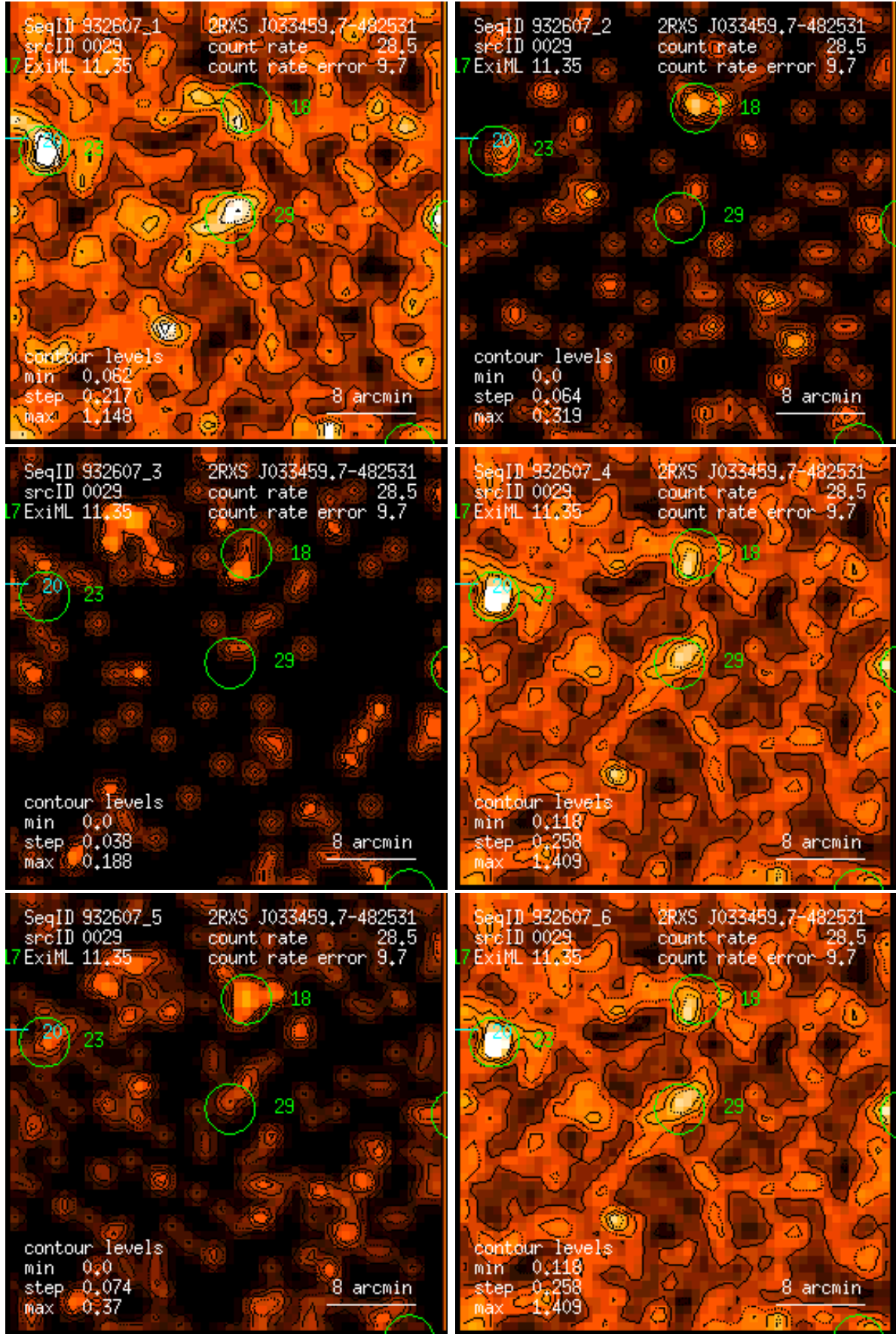
Figure 29: RASS 932607: detection 0029: band rate images, Gaussian filter: (1) PSPC channels 11 – 41, (2) 52 – 90, (3) 91 – 201, (4) 11 – 235, (5) 52 – 201, (6) 11 – 201. Broad band rates in counts/ks. Band rate contour levels in counts/ks/arcmin 2 .
