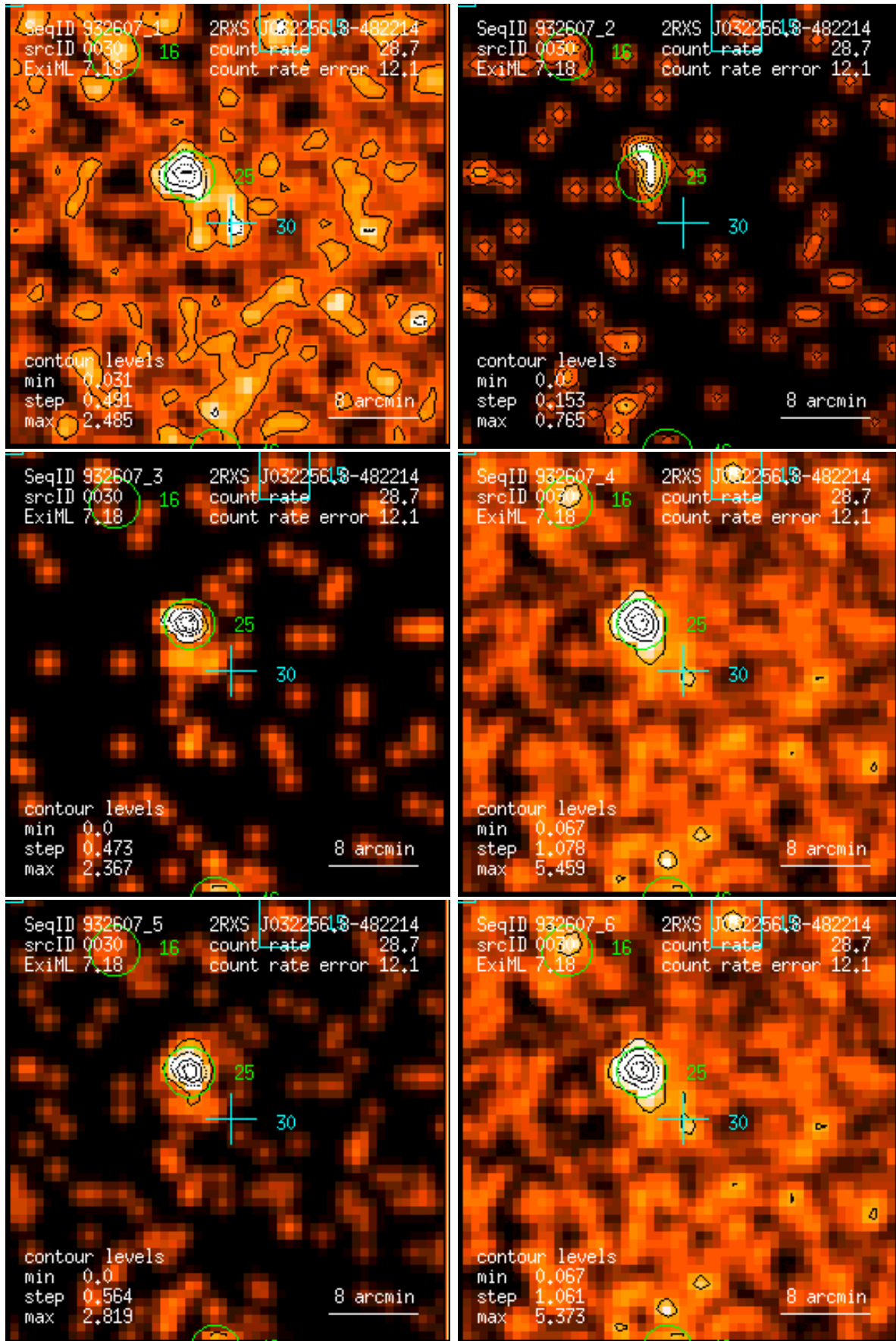
Figure 30: RASS 932607: detection 0030: band rate images, Gaussian filter: (1) PSPC channels 11 – 41, (2) 52 – 90, (3) 91 – 201, (4) 11 – 235, (5) 52 – 201, (6) 11 – 201. Broad band rates in counts/ks. Band rate contour levels in counts/ks/arcmin 2 .
