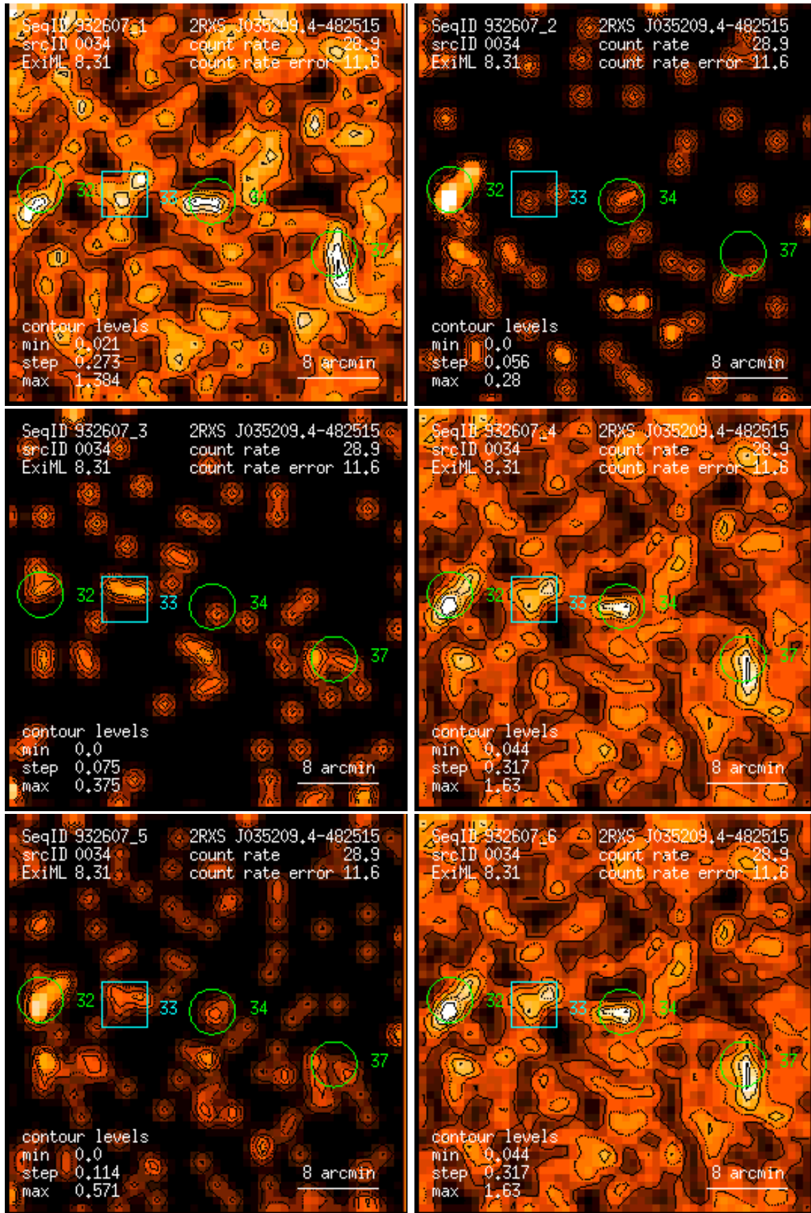
Figure 34: RASS 932607: detection 0034: band rate images, Gaussian filter: (1) PSPC channels 11 – 41, (2) 52 – 90, (3) 91 – 201, (4) 11 – 235, (5) 52 – 201, (6) 11 – 201. Broad band rates in counts/ks. Band rate contour levels in counts/ks/arcmin 2 .
